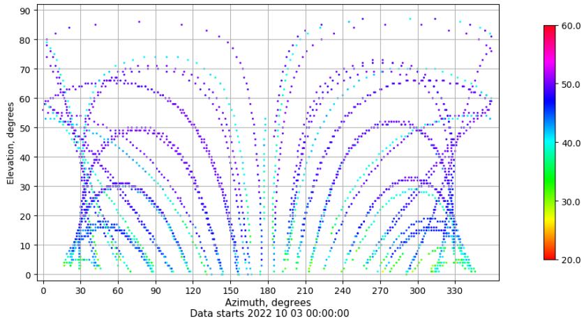
Azimuth-elevation plot for station ZFRA. Signal to Noise S1C Data file ZFRA00ESP_R_2022276.xtr
