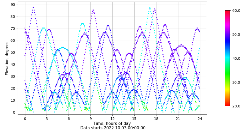
Time-elevation plot for station ZFRA. Signal to Noise S1C Data file ZFRA00ESP_R_2022276.xtr
