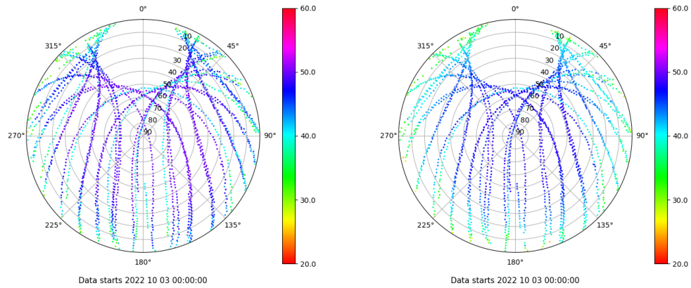
Skyplot for station ZFRA. Signal to Noise S1C Data file ZFRA00ESP_R_2022276.xtr Skyplot for station ZFRA. Signal to Noise S2P Data file ZFRA00ESP_R_2022276.xtr
