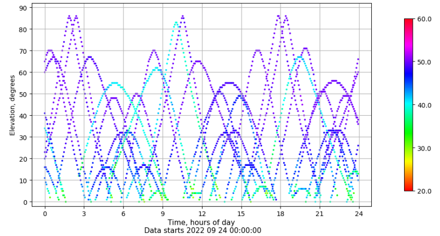
Time-elevation plot for station ZFRA. Signal to Noise S1C Data file ZFRA00ESP_R_2022267.xtr
