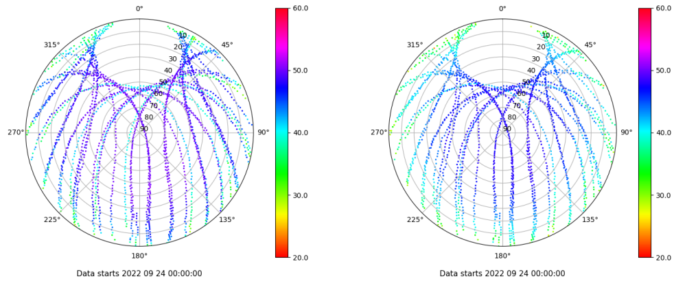
Skyplot for station ZFRA. Signal to Noise S1C Data file ZFRA00ESP_R_2022267.xtr Skyplot for station ZFRA. Signal to Noise S2P Data file ZFRA00ESP_R_2022267.xtr
