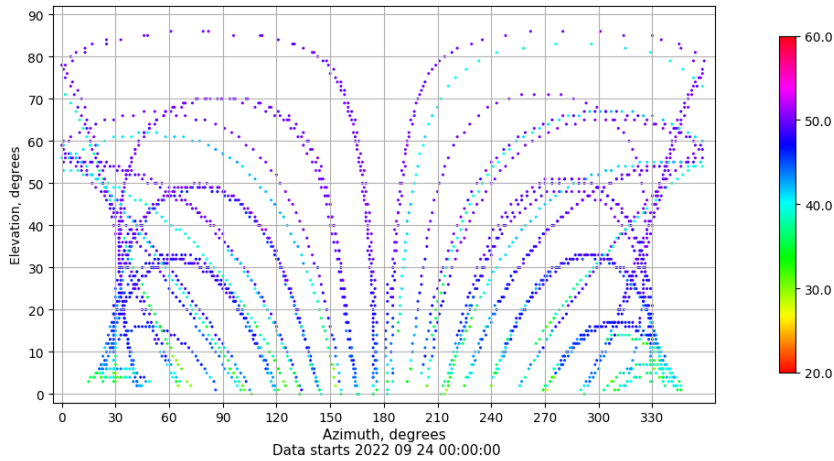
Azimuth-elevation plot for station ZFRA. Signal to Noise S1C Data file ZFRA00ESP_R_2022267.xtr
