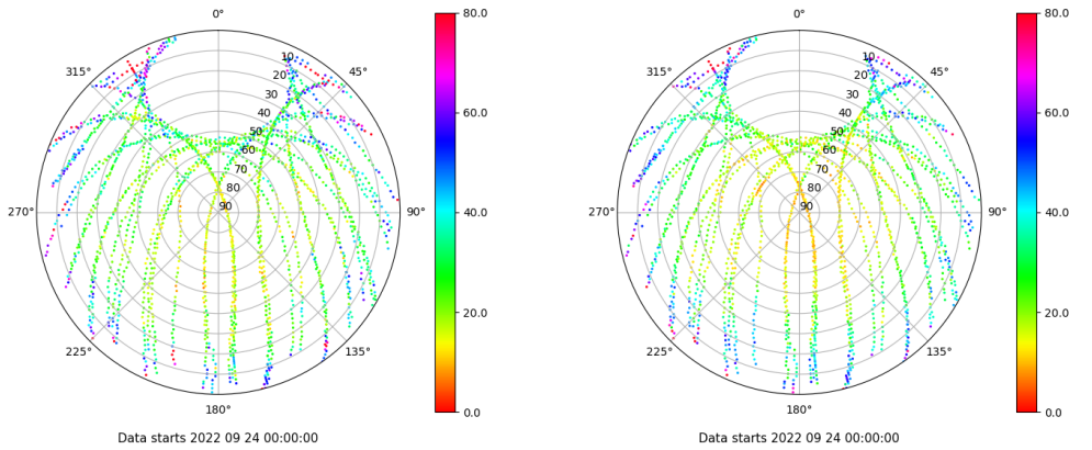
Skyplot for station ZFRA. Parameter M1C Data file ZFRA00ESP_R_2022267.xtr Skyplot for station ZFRA. Parameter M2P Data file ZFRA00ESP_R_2022267.xtr
