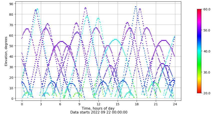
Time-elevation plot for station ZFRA. Signal to Noise S1C Data file ZFRA00ESP_R_2022265.xtr
