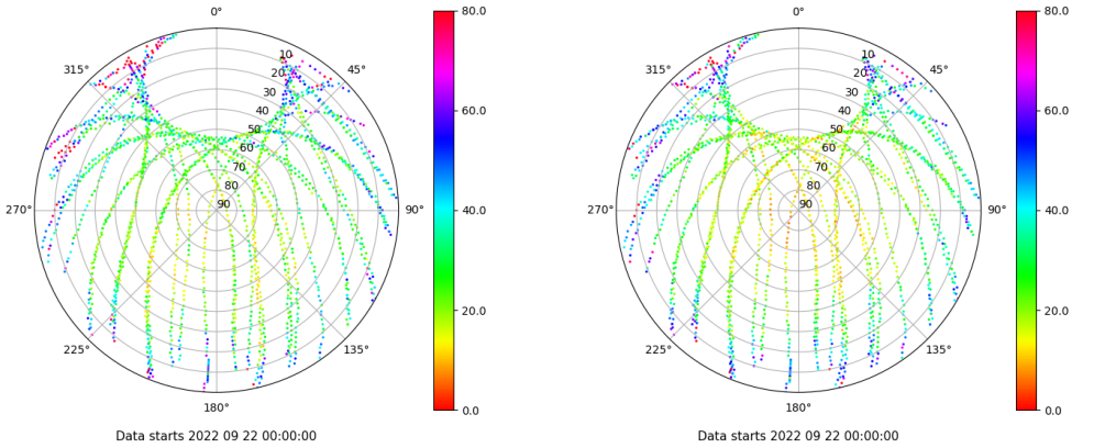
Skyplot for station ZFRA. Parameter M1C Data file ZFRA00ESP_R_2022265.xtr Skyplot for station ZFRA. Parameter M2P Data file ZFRA00ESP_R_2022265.xtr
