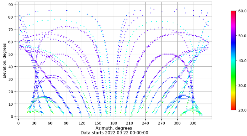
Azimuth-elevation plot for station ZFRA. Signal to Noise S1C Data file ZFRA00ESP_R_2022265.xtr
