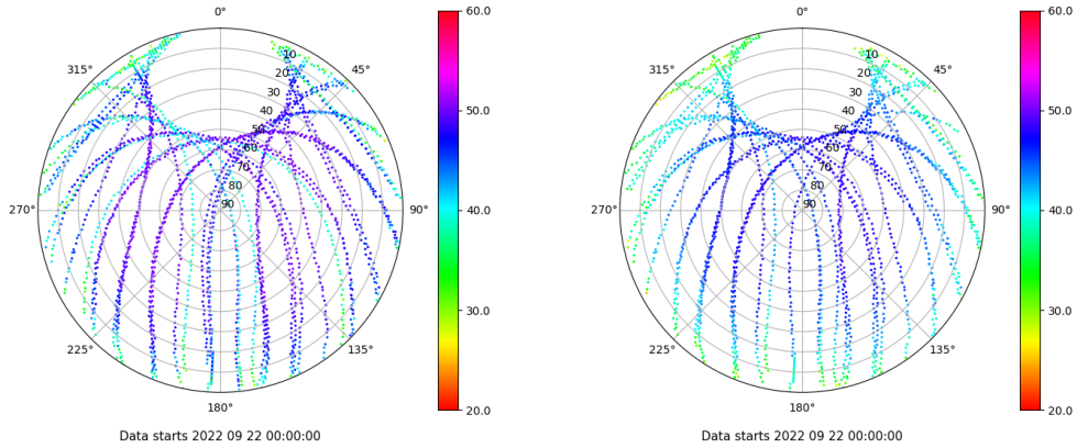
Skyplot for station ZFRA. Signal to Noise S1C Data file ZFRA00ESP_R_2022265.xtr Skyplot for station ZFRA. Signal to Noise S2P Data file ZFRA00ESP_R_2022265.xtr
