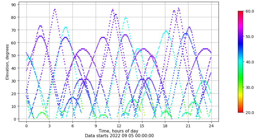
Time-elevation plot for station ZFRA. Signal to Noise S1C Data file ZFRA00ESP_R_2022248.xtr
