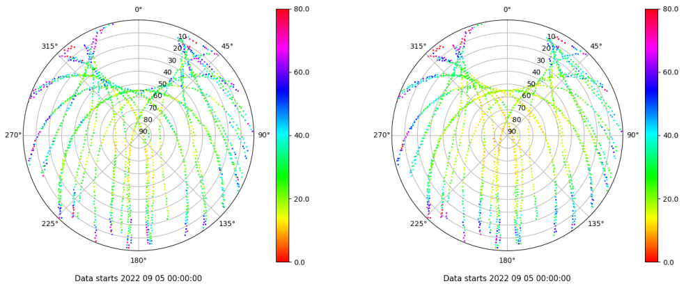
Skyplot for station ZFRA. Parameter M1C Data file ZFRA00ESP_R_2022248.xtr Skyplot for station ZFRA. Parameter M2P Data file ZFRA00ESP_R_2022248.xtr
