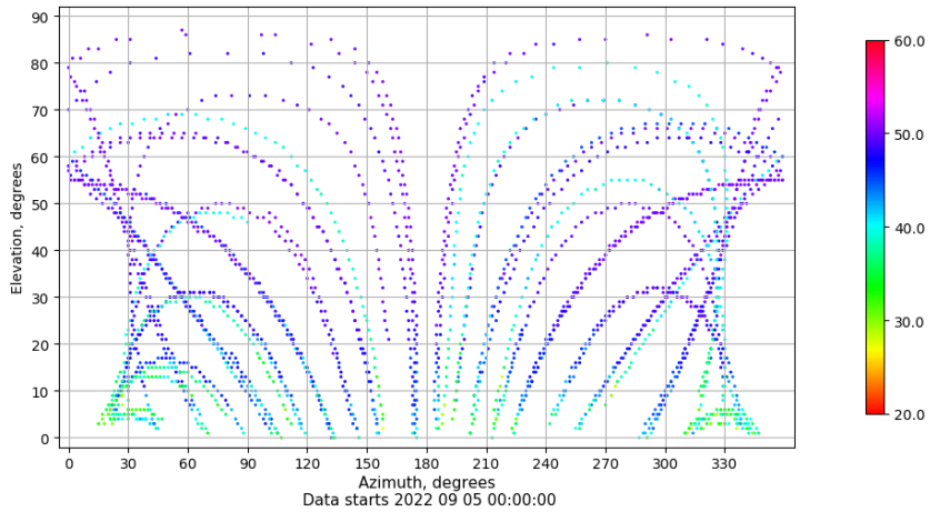
Azimuth-elevation plot for station ZFRA. Signal to Noise S1C Data file ZFRA00ESP_R_2022248.xtr
