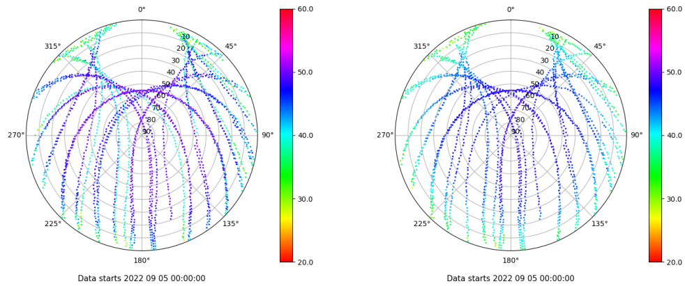
Skyplot for station ZFRA. Signal to Noise S1C Data file ZFRA00ESP_R_2022248.xtr Skyplot for station ZFRA. Signal to Noise S2P Data file ZFRA00ESP_R_2022248.xtr
