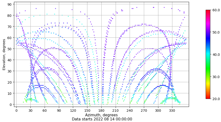
Azimuth-elevation plot for station ZFRA. Signal to Noise S1C Data file ZFRA00ESP_R_20222226.xtr
