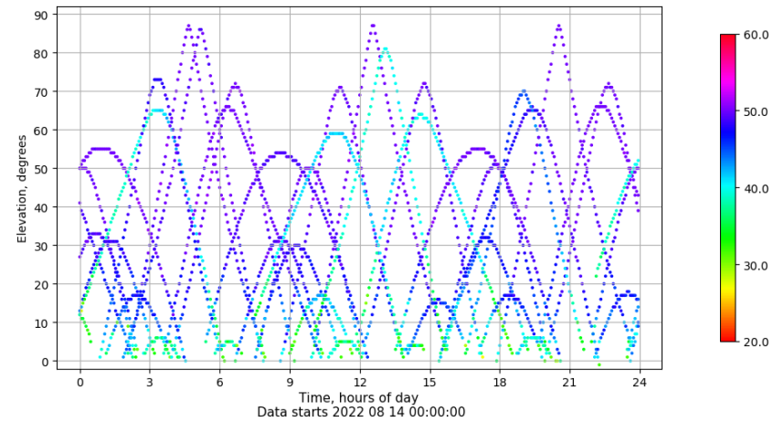
Time-elevation plot for station ZFRA. Signal to Noise S1C Data file ZFRA00ESP_R_20222226.xtr
