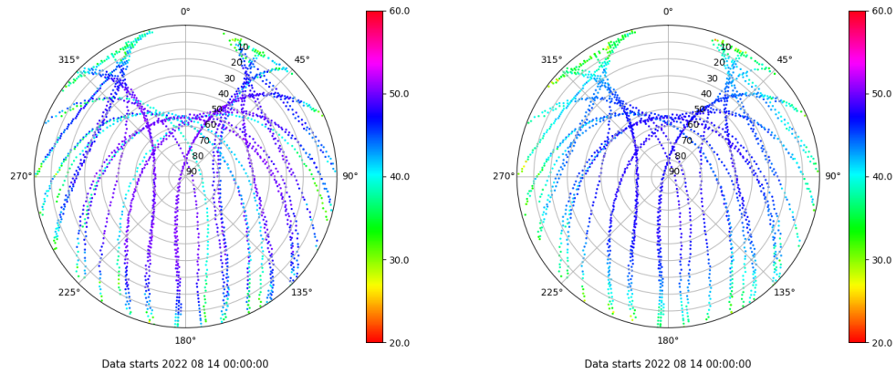
Skyplot for station ZFRA. Signal to Noise S1C Data file ZFRA00ESP_R_20222226.xtr Skyplot for station ZFRA. Signal to Noise S2P Data file ZFRA00ESP_R_20222226.xtr
