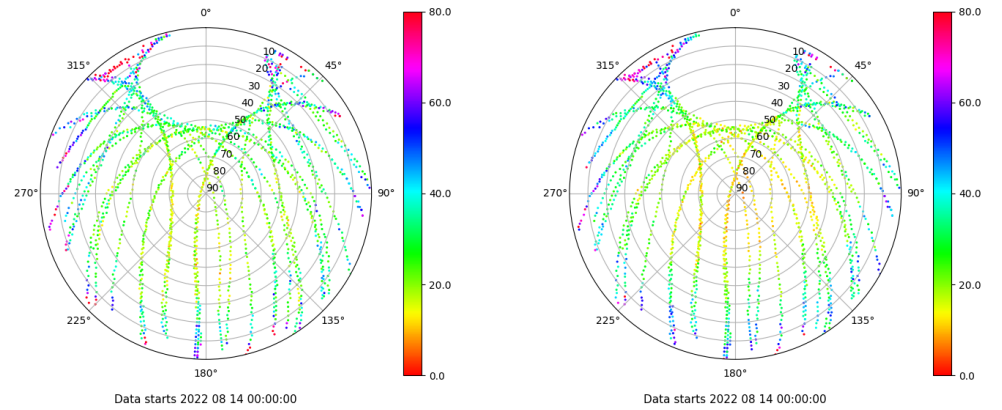
Skyplot for station ZFRA. Parameter M1C Data file ZFRA00ESP_R_20222226.xtr Skyplot for station ZFRA. Parameter M2P Data file ZFRA00ESP_R_20222226.xtr
