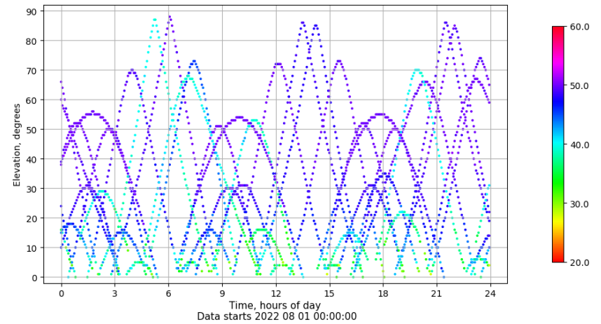
Time-elevation plot for station ZFRA. Signal to Noise S1C Data file ZFRA00ESP_R_2022213.xtr
