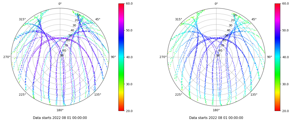
Skyplot for station ZFRA. Signal to Noise S1C Data file ZFRA00ESP_R_2022213.xtr Skyplot for station ZFRA. Signal to Noise S2P Data file ZFRA00ESP_R_2022213.xtr
