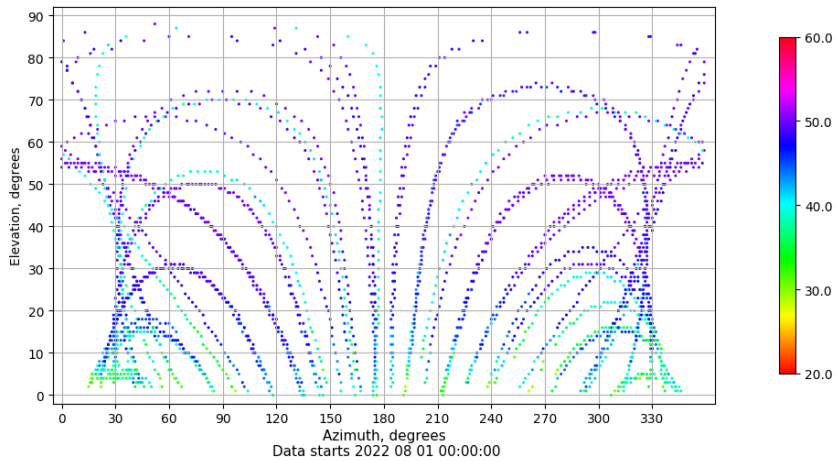
Azimuth-elevation plot for station ZFRA. Signal to Noise S1C Data file ZFRA00ESP_R_2022213.xtr
