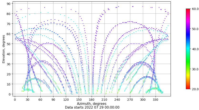
Azimuth-elevation plot for station ZFRA. Signal to Noise S1C Data file ZFRA00ESP_R_2022210.xtr
