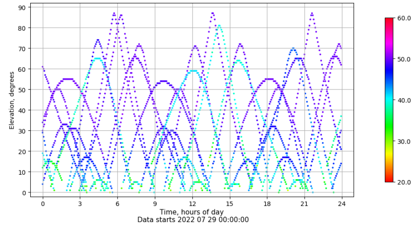
Time-elevation plot for station ZFRA. Signal to Noise S1C Data file ZFRA00ESP_R_2022210.xtr
