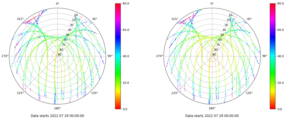
Skyplot for station ZFRA. Parameter M1C Data file ZFRA00ESP_R_2022210.xtr Skyplot for station ZFRA. Parameter M2P Data file ZFRA00ESP_R_2022210.xtr
