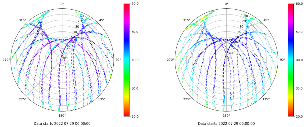
Skyplot for station ZFRA. Signal to Noise S1C Data file ZFRA00ESP_R_2022210.xtr Skyplot for station ZFRA. Signal to Noise S2P Data file ZFRA00ESP_R_2022210.xtr
