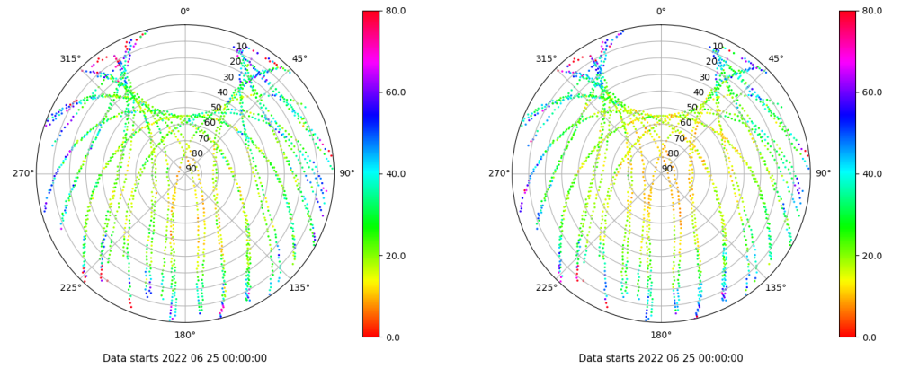
Skyplot for station ZFRA. Parameter M1C Data file ZFRA00ESP_R_2022176.xtr Skyplot for station ZFRA. Parameter M2P Data file ZFRA00ESP_R_2022176.xtr
