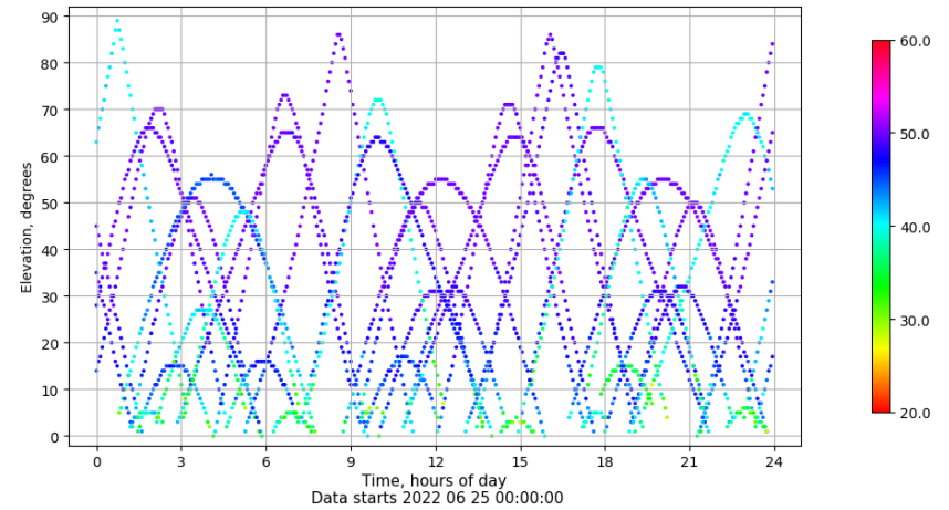
Time-elevation plot for station ZFRA. Signal to Noise S1C Data file ZFRA00ESP_R_2022176.xtr
