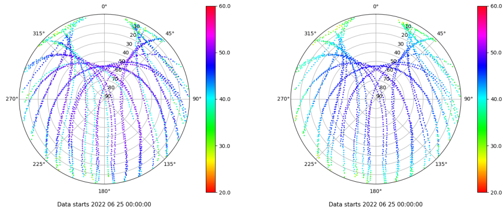
Skyplot for station ZFRA. Signal to Noise S1C Data file ZFRA00ESP_R_2022176.xtr Skyplot for station ZFRA. Signal to Noise S2P Data file ZFRA00ESP_R_2022176.xtr
