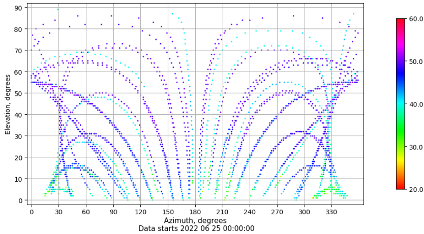
Azimuth-elevation plot for station ZFRA. Signal to Noise S1C Data file ZFRA00ESP_R_2022176.xtr
