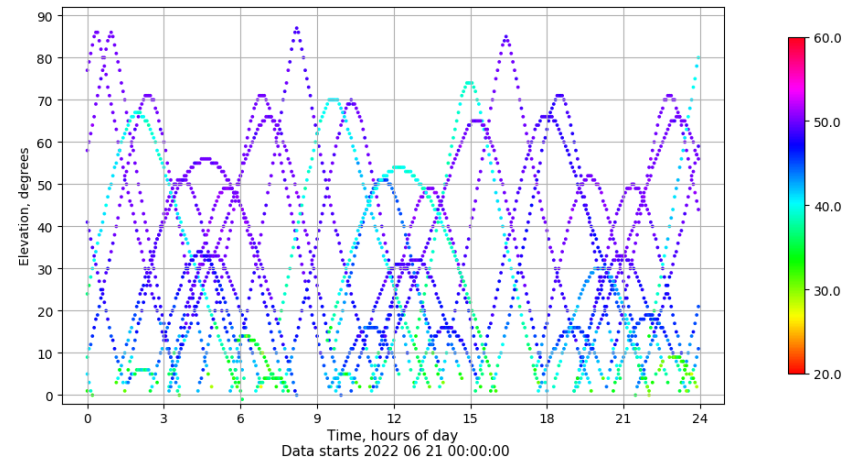
Time-elevation plot for station ZFRA. Signal to Noise S1C Data file ZFRA00ESP_R_2022172.xtr
