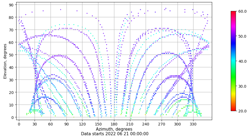
Azimuth-elevation plot for station ZFRA. Signal to Noise S1C Data file ZFRA00ESP_R_2022172.xtr
