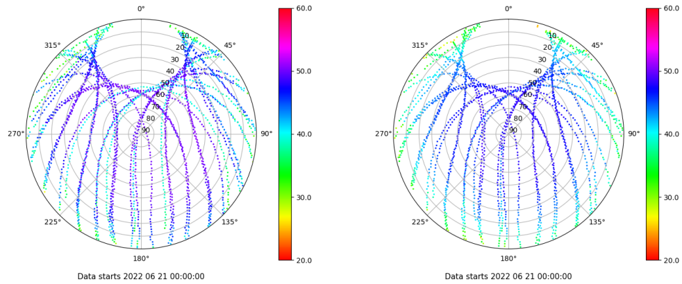
Skyplot for station ZFRA. Signal to Noise S1C Data file ZFRA00ESP_R_2022172.xtr Skyplot for station ZFRA. Signal to Noise S2P Data file ZFRA00ESP_R_2022172.xtr
