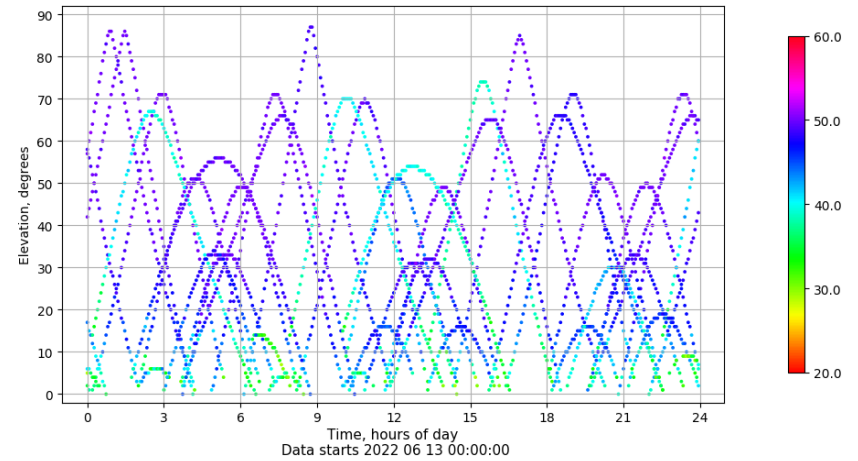
Time-elevation plot for station ZFRA. Signal to Noise S1C Data file ZFRA00ESP_R_2022164.xtr
