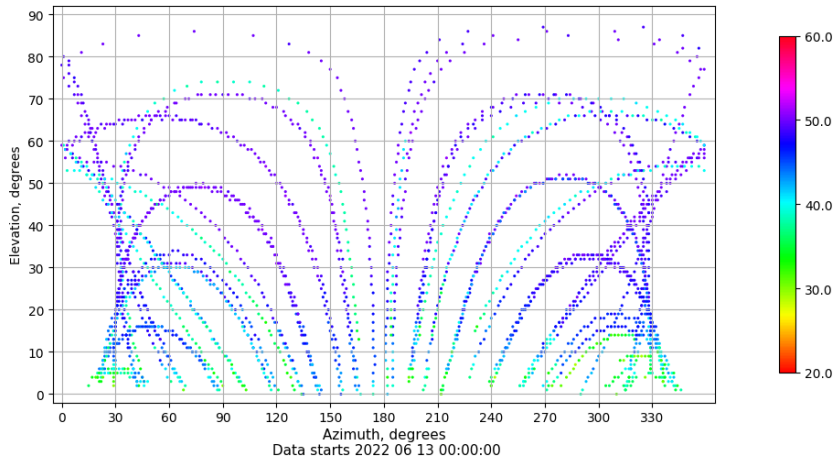
Azimuth-elevation plot for station ZFRA. Signal to Noise S1C Data file ZFRA00ESP_R_2022164.xtr
