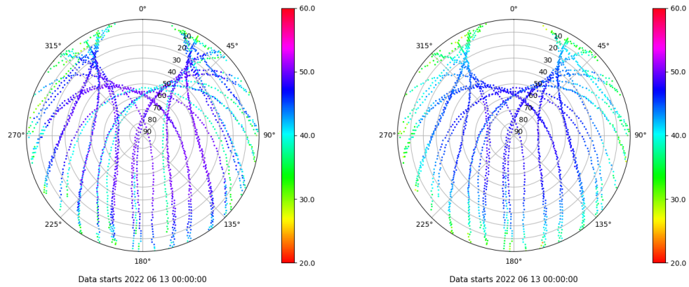
Skyplot for station ZFRA. Signal to Noise S1C Data file ZFRA00ESP_R_2022164.xtr Skyplot for station ZFRA. Signal to Noise S2P Data file ZFRA00ESP_R_2022164.xtr
