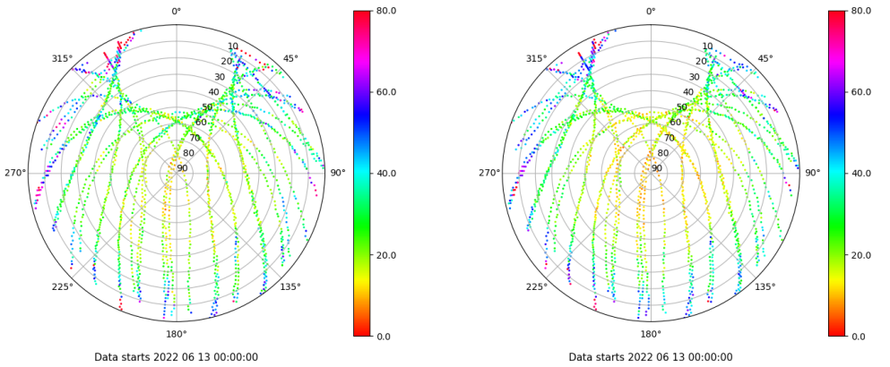
Skyplot for station ZFRA. Parameter M1C Data file ZFRA00ESP_R_2022164.xtr Skyplot for station ZFRA. Parameter M2P Data file ZFRA00ESP_R_2022164.xtr
