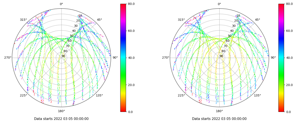
Skyplot for station ZFRA. Parameter M1C Data file ZFRA00ESP_R_2022064.xtr Skyplot for station ZFRA. Parameter M2P Data file ZFRA00ESP_R_2022064.xtr
