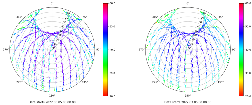
Skyplot for station ZFRA. Signal to Noise S1C Data file ZFRA00ESP_R_2022064.xtr Skyplot for station ZFRA. Signal to Noise S2P Data file ZFRA00ESP_R_2022064.xtr
