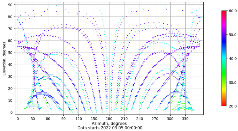
Azimuth-elevation plot for station ZFRA. Signal to Noise S1C Data file ZFRA00ESP_R_2022064.xtr
