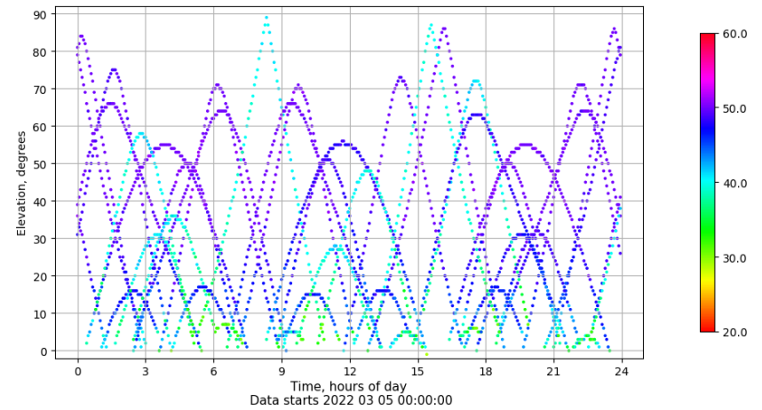
Time-elevation plot for station ZFRA. Signal to Noise S1C Data file ZFRA00ESP_R_2022064.xtr
