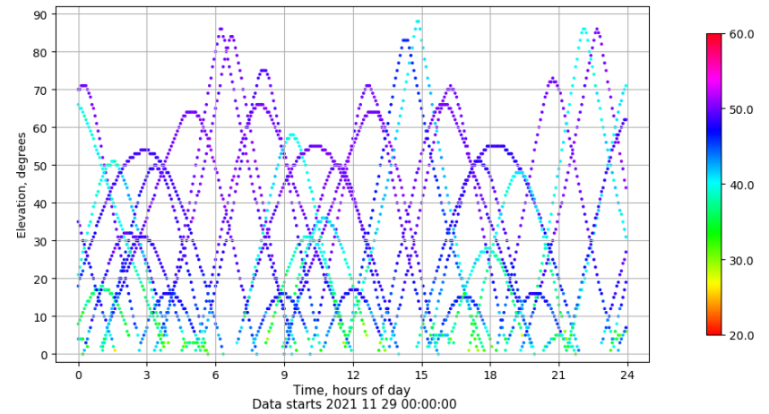
Time-elevation plot for station ZFRA. Signal to Noise S1C Data file ZFRA00ESP_R_2021333.xtr
