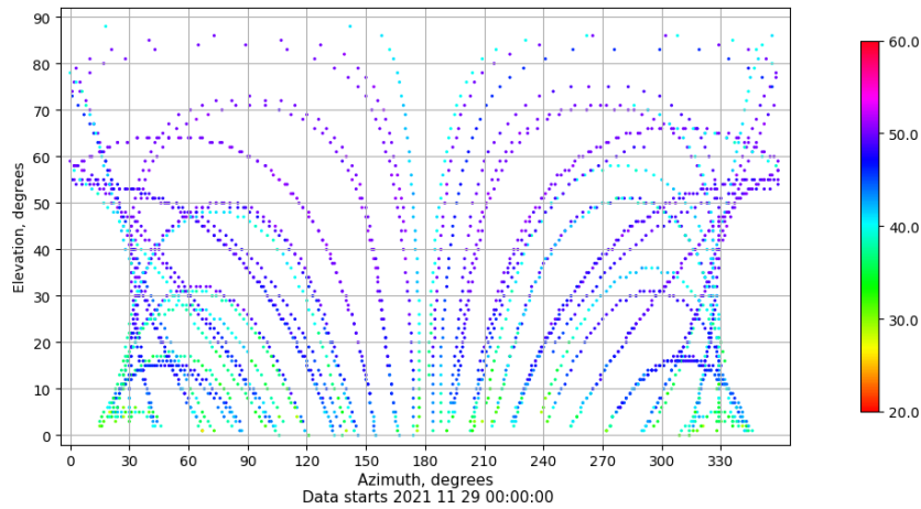
Azimuth-elevation plot for station ZFRA. Signal to Noise S1C Data file ZFRA00ESP_R_2021333.xtr
