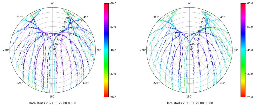
Skyplot for station ZFRA. Signal to Noise S1C Data file ZFRA00ESP_R_2021333.xtr Skyplot for station ZFRA. Signal to Noise S2P Data file ZFRA00ESP_R_2021333.xtr
