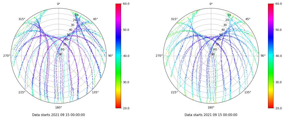
Skyplot for station ZFRA. Signal to Noise S1C Data file ZFRA00ESP_R_2021258.xtr Skyplot for station ZFRA. Signal to Noise S2P Data file ZFRA00ESP_R_2021258.xtr
