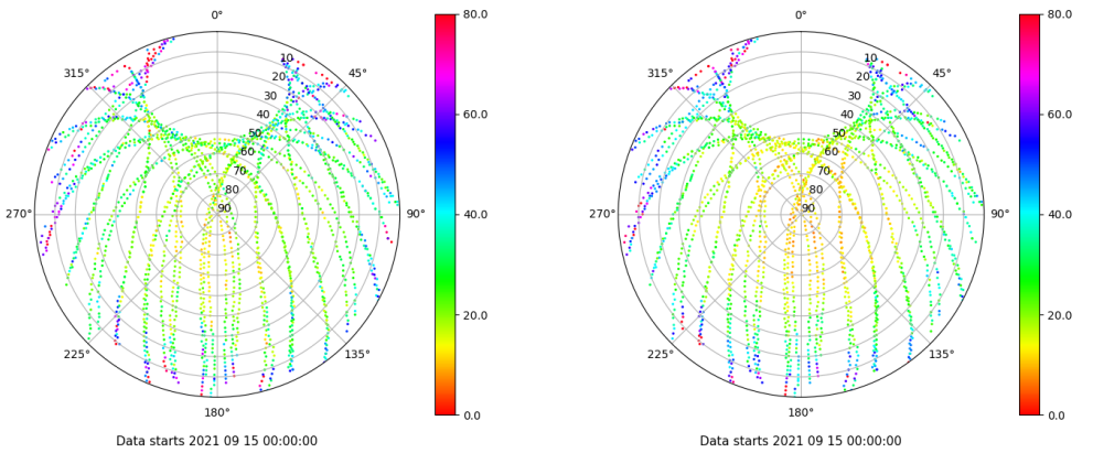
Skyplot for station ZFRA. Parameter M1C Data file ZFRA00ESP_R_2021258.xtr Skyplot for station ZFRA. Parameter M2P Data file ZFRA00ESP_R_2021258.xtr
