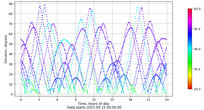
Time-elevation plot for station ZFRA. Signal to Noise S1C Data file ZFRA00ESP_R_2021258.xtr
