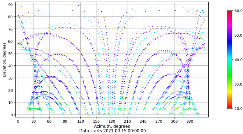
Azimuth-elevation plot for station ZFRA. Signal to Noise S1C Data file ZFRA00ESP_R_2021258.xtr
