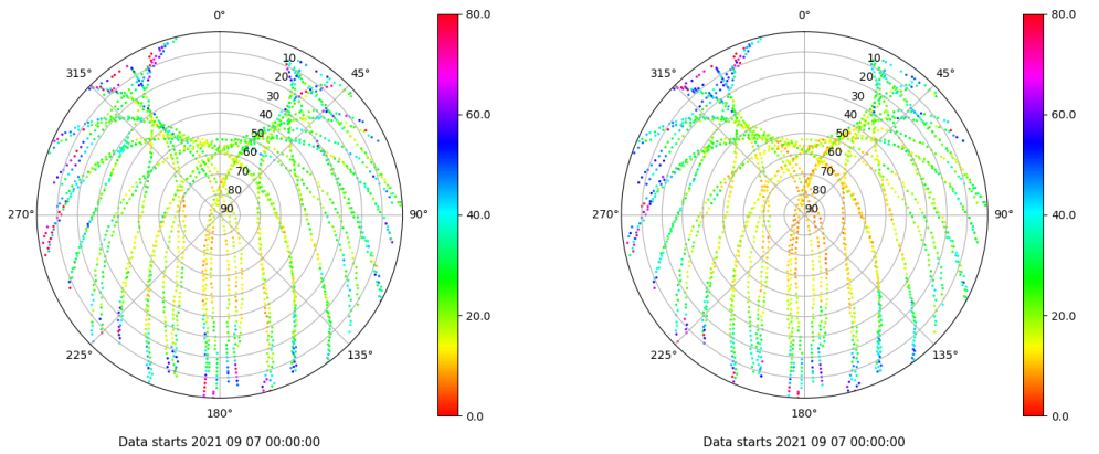
Skyplot for station ZFRA. Parameter M1C Data file ZFRA00ESP_R_2021250.xtr Skyplot for station ZFRA. Parameter M2P Data file ZFRA00ESP_R_2021250.xtr
