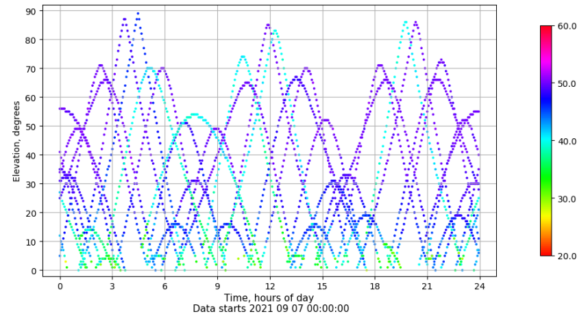
Time-elevation plot for station ZFRA. Signal to Noise S1C Data file ZFRA00ESP_R_2021250.xtr
