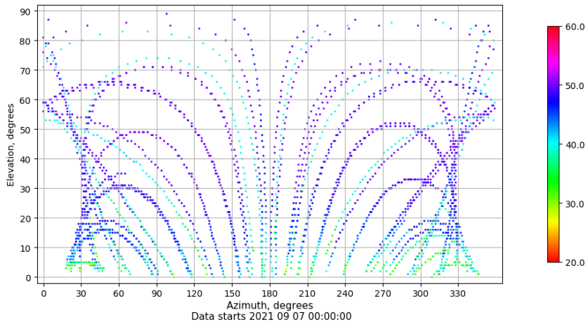
Azimuth-elevation plot for station ZFRA. Signal to Noise S1C Data file ZFRA00ESP_R_2021250.xtr
