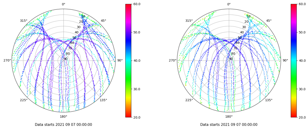
Skyplot for station ZFRA. Signal to Noise S1C Data file ZFRA00ESP_R_2021250.xtr Skyplot for station ZFRA. Signal to Noise S2P Data file ZFRA00ESP_R_2021250.xtr
