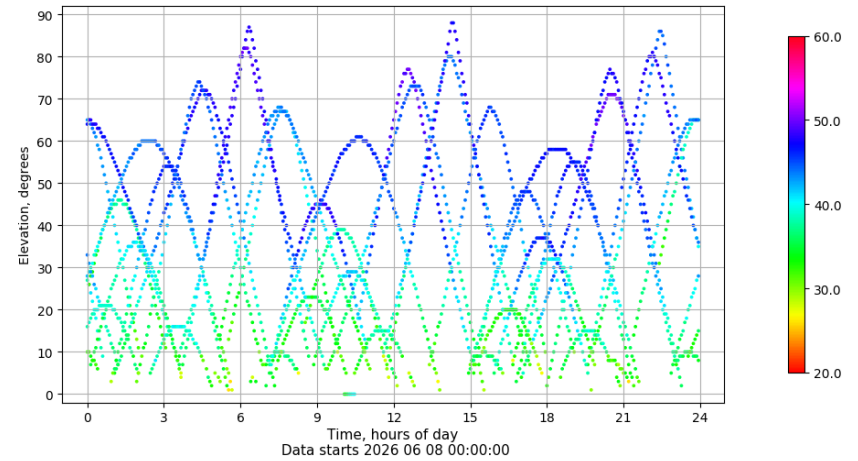
Time-elevation plot for station ZARA. Signal to Noise S1C Data file ZARA00ESP_R_2026159.xtr
