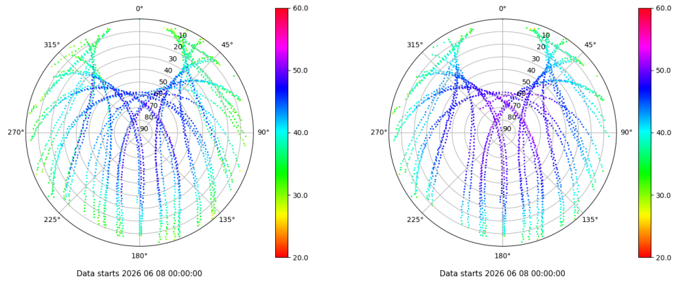
Skyplot for station ZARA. Signal to Noise S1C Data file ZARA00ESP_R_2026159.xtr Skyplot for station ZARA. Signal to Noise S2C Data file ZARA00ESP_R_2026159.xtr
