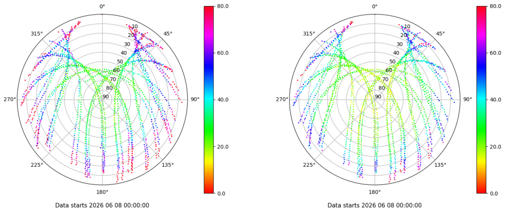
Skyplot for station ZARA. Parameter M1C Data file ZARA00ESP_R_2026159.xtr Skyplot for station ZARA. Parameter M2C Data file ZARA00ESP_R_2026159.xtr
