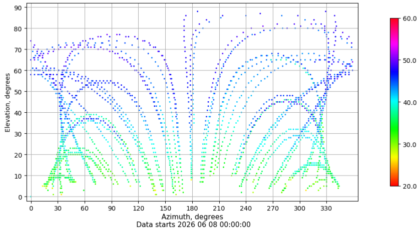
Azimuth-elevation plot for station ZARA. Signal to Noise S1C Data file ZARA00ESP_R_2026159.xtr
