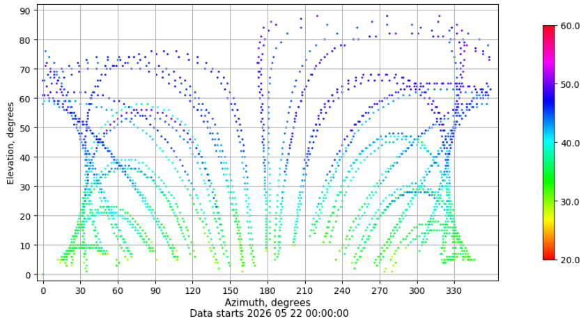
Azimuth-elevation plot for station ZARA. Signal to Noise S1C Data file ZARA00ESP_R_2026142.xtr
