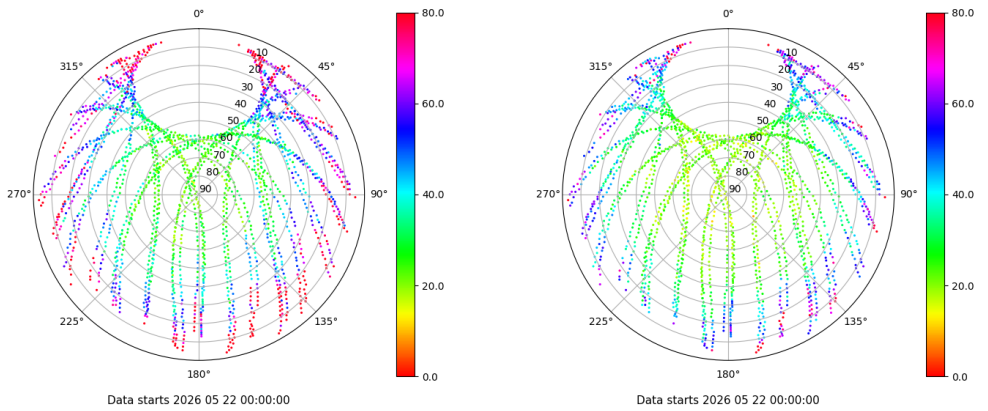
Skyplot for station ZARA. Parameter M1C Data file ZARA00ESP_R_2026142.xtr Skyplot for station ZARA. Parameter M2C Data file ZARA00ESP_R_2026142.xtr
