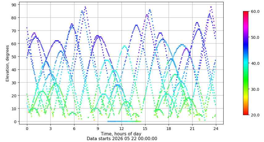
Time-elevation plot for station ZARA. Signal to Noise S1C Data file ZARA00ESP_R_2026142.xtr
