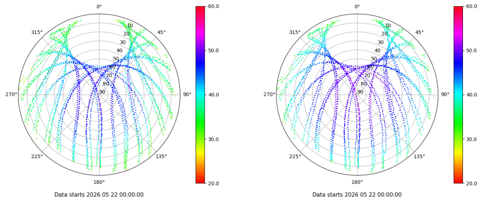
Skyplot for station ZARA. Signal to Noise S1C Data file ZARA00ESP_R_2026142.xtr Skyplot for station ZARA. Signal to Noise S2C Data file ZARA00ESP_R_2026142.xtr
