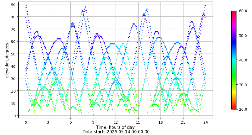
Time-elevation plot for station ZARA. Signal to Noise S1C Data file ZARA00ESP_R_2026134.xtr
