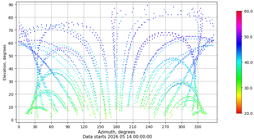
Azimuth-elevation plot for station ZARA. Signal to Noise S1C Data file ZARA00ESP_R_2026134.xtr
