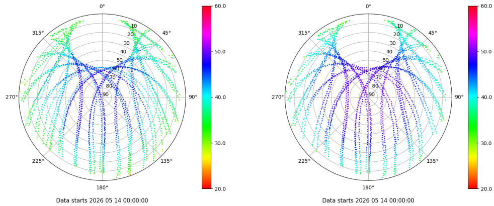
Skyplot for station ZARA. Signal to Noise S1C Data file ZARA00ESP_R_2026134.xtr Skyplot for station ZARA. Signal to Noise S2C Data file ZARA00ESP_R_2026134.xtr
