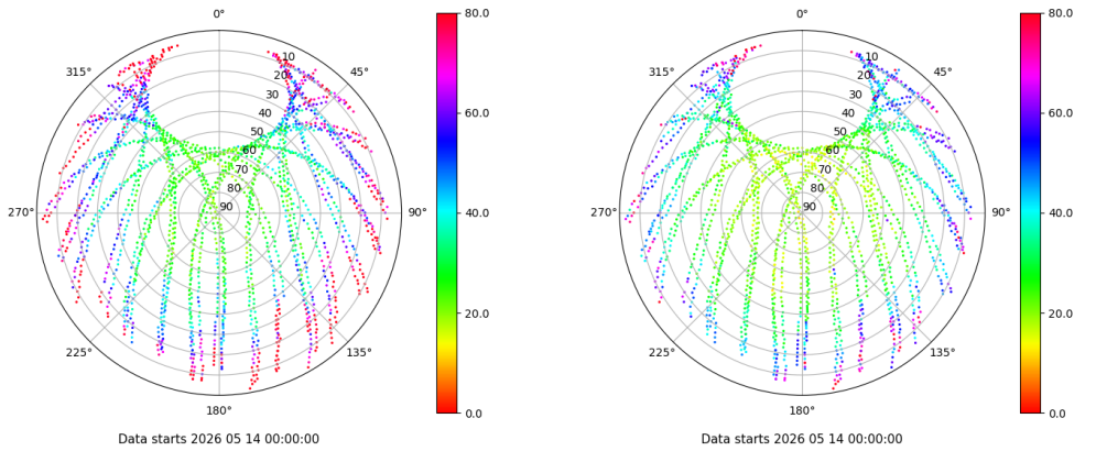
Skyplot for station ZARA. Parameter M1C Data file ZARA00ESP_R_2026134.xtr Skyplot for station ZARA. Parameter M2C Data file ZARA00ESP_R_2026134.xtr
