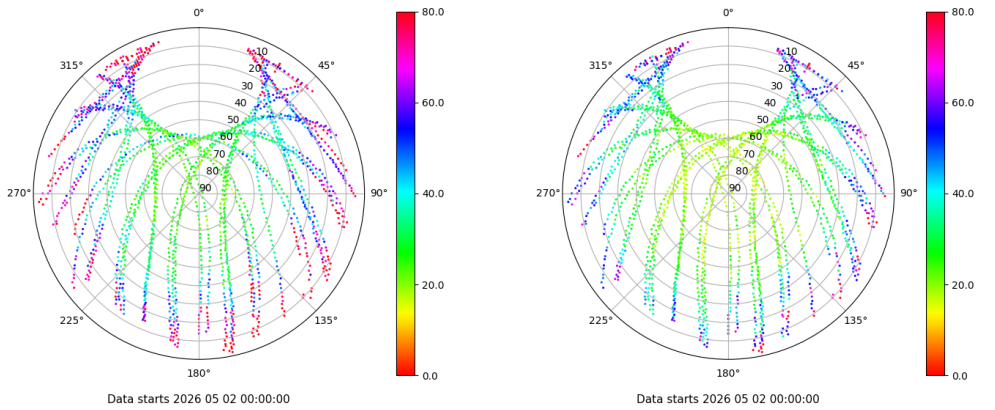
Skyplot for station ZARA. Parameter M1C Data file ZARA00ESP_R_2026122.xtr Skyplot for station ZARA. Parameter M2C Data file ZARA00ESP_R_2026122.xtr
