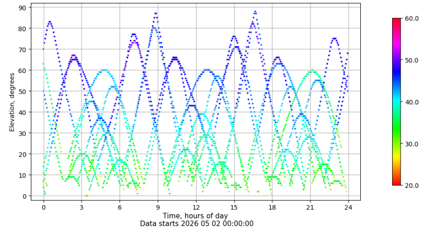
Time-elevation plot for station ZARA. Signal to Noise S1C Data file ZARA00ESP_R_2026122.xtr
