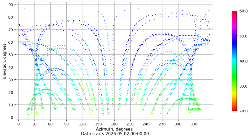
Azimuth-elevation plot for station ZARA. Signal to Noise S1C Data file ZARA00ESP_R_2026122.xtr
