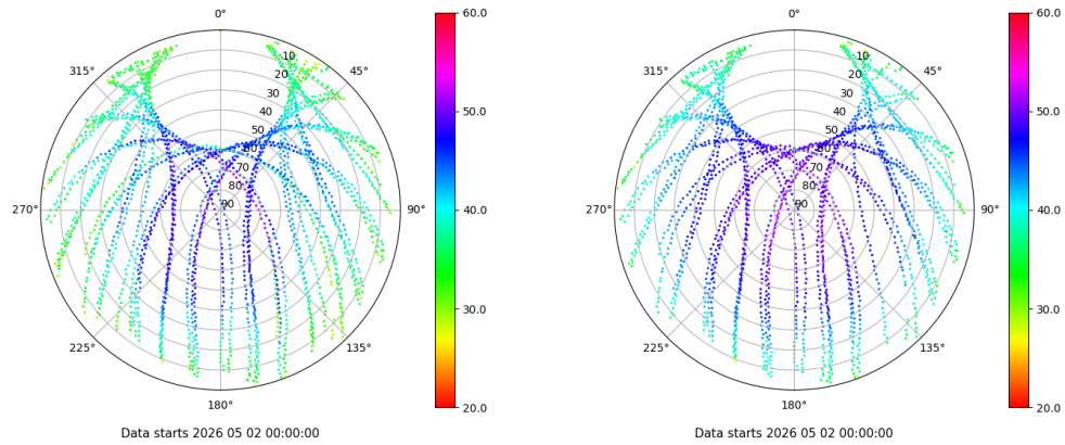
Skyplot for station ZARA. Signal to Noise S1C Data file ZARA00ESP_R_2026122.xtr Skyplot for station ZARA. Signal to Noise S2C Data file ZARA00ESP_R_2026122.xtr
