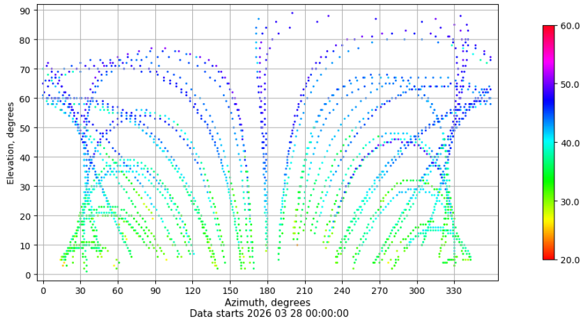
Azimuth-elevation plot for station ZARA. Signal to Noise S1C Data file ZARA00ESP_R_2026087.xtr
