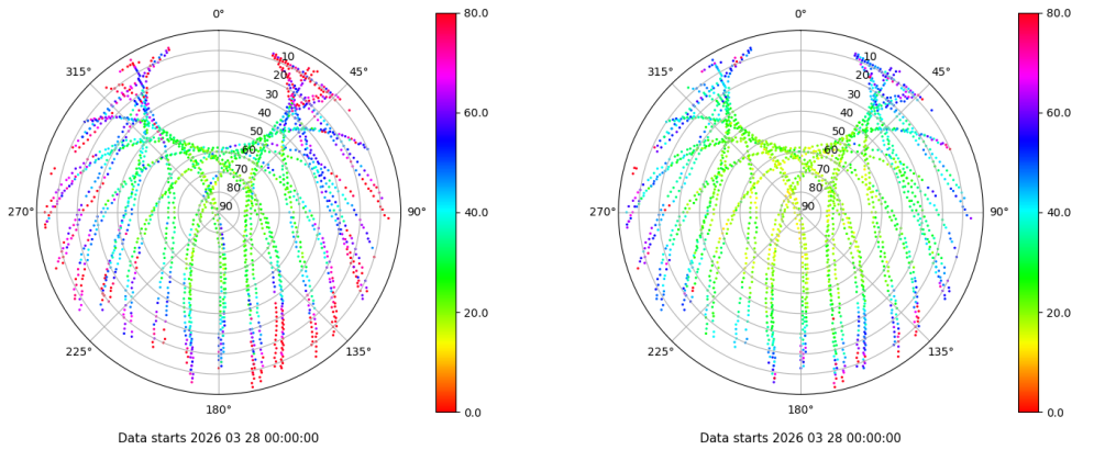
Skyplot for station ZARA. Parameter M1C Data file ZARA00ESP_R_2026087.xtr Skyplot for station ZARA. Parameter M2C Data file ZARA00ESP_R_2026087.xtr
