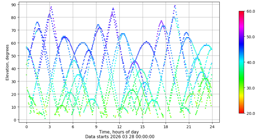
Time-elevation plot for station ZARA. Signal to Noise S1C Data file ZARA00ESP_R_2026087.xtr
