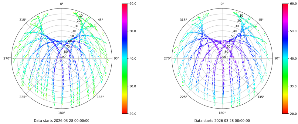
Skyplot for station ZARA. Signal to Noise S1C Data file ZARA00ESP_R_2026087.xtr Skyplot for station ZARA. Signal to Noise S2C Data file ZARA00ESP_R_2026087.xtr
