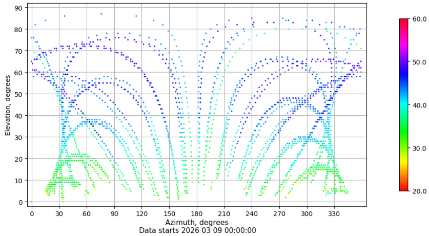
Azimuth-elevation plot for station ZARA. Signal to Noise S1C Data file ZARA00ESP_R_2026068.xtr
