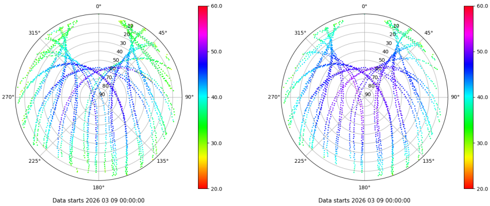
Skyplot for station ZARA. Signal to Noise S1C Data file ZARA00ESP_R_2026068.xtr Skyplot for station ZARA. Signal to Noise S2C Data file ZARA00ESP_R_2026068.xtr
