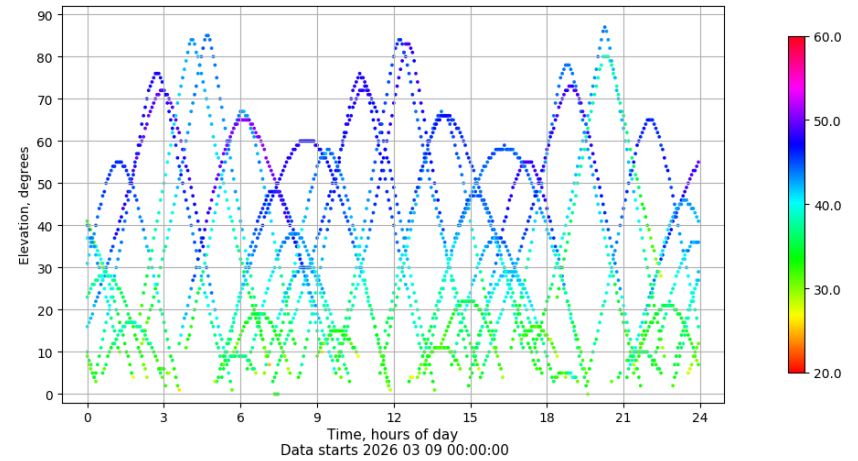
Time-elevation plot for station ZARA. Signal to Noise S1C Data file ZARA00ESP_R_2026068.xtr
