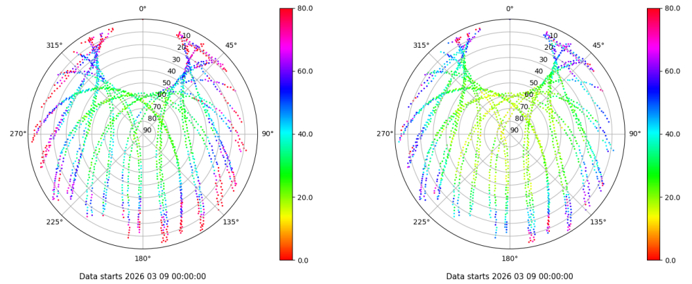
Skyplot for station ZARA. Parameter M1C Data file ZARA00ESP_R_2026068.xtr Skyplot for station ZARA. Parameter M2C Data file ZARA00ESP_R_2026068.xtr
