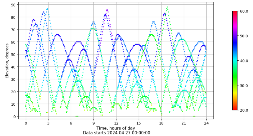
Time-elevation plot for station ZARA. Signal to Noise S1C Data file ZARA00ESP_R_2024118.xtr
