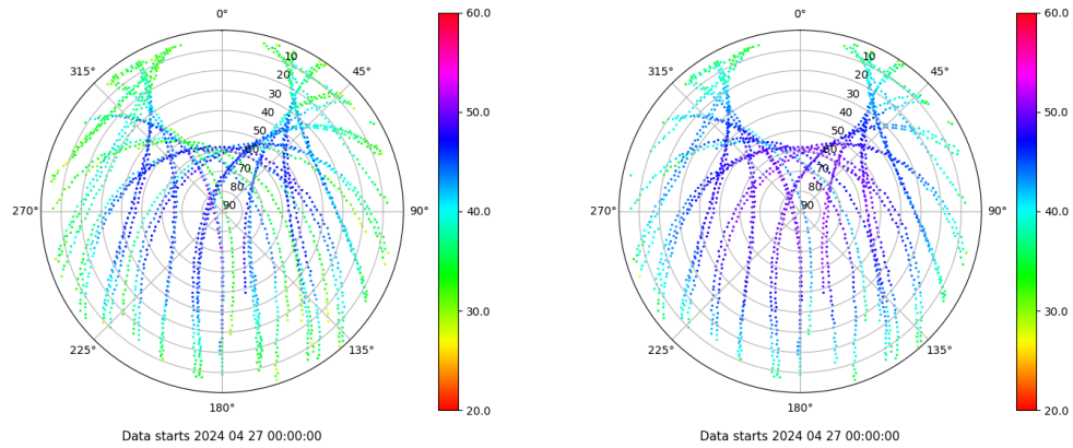
Skyplot for station ZARA. Signal to Noise S1C Data file ZARA00ESP_R_2024118.xtr Skyplot for station ZARA. Signal to Noise S2C Data file ZARA00ESP_R_2024118.xtr
