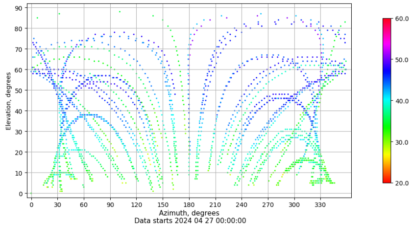
Azimuth-elevation plot for station ZARA. Signal to Noise S1C Data file ZARA00ESP_R_2024118.xtr
