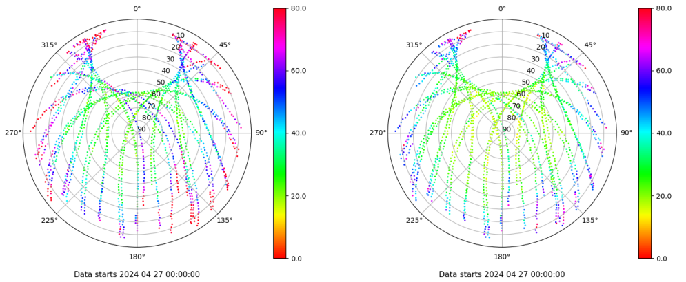
Skyplot for station ZARA. Parameter M1C Data file ZARA00ESP_R_2024118.xtr Skyplot for station ZARA. Parameter M2C Data file ZARA00ESP_R_2024118.xtr
