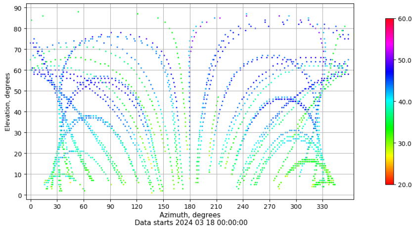
Azimuth-elevation plot for station ZARA. Signal to Noise S1C Data file ZARA00ESP_R_2024078.xtr
