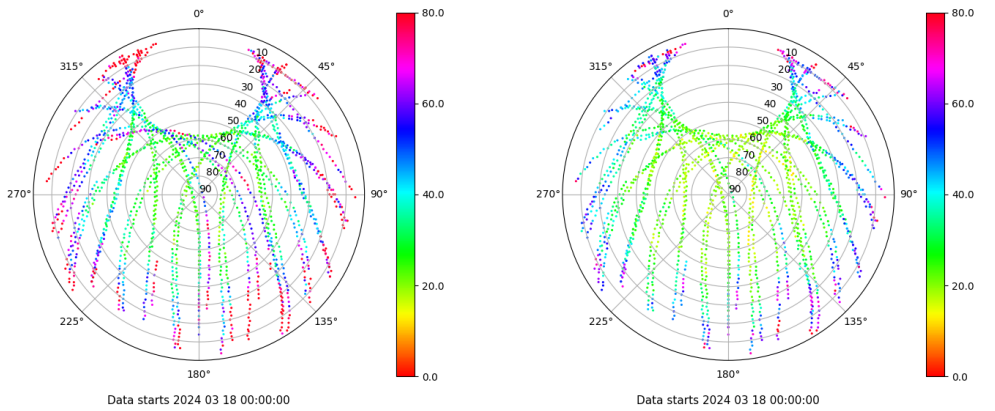
Skyplot for station ZARA. Parameter M1C Data file ZARA00ESP_R_2024078.xtr Skyplot for station ZARA. Parameter M2C Data file ZARA00ESP_R_2024078.xtr
