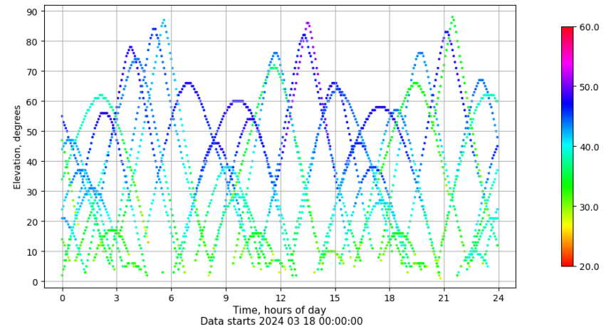
Time-elevation plot for station ZARA. Signal to Noise S1C Data file ZARA00ESP_R_2024078.xtr
