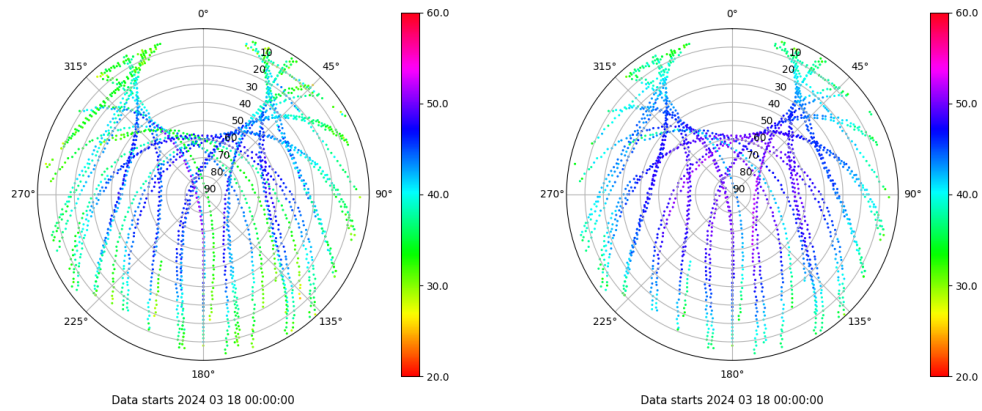
Skyplot for station ZARA. Signal to Noise S1C Data file ZARA00ESP_R_2024078.xtr Skyplot for station ZARA. Signal to Noise S2C Data file ZARA00ESP_R_2024078.xtr
