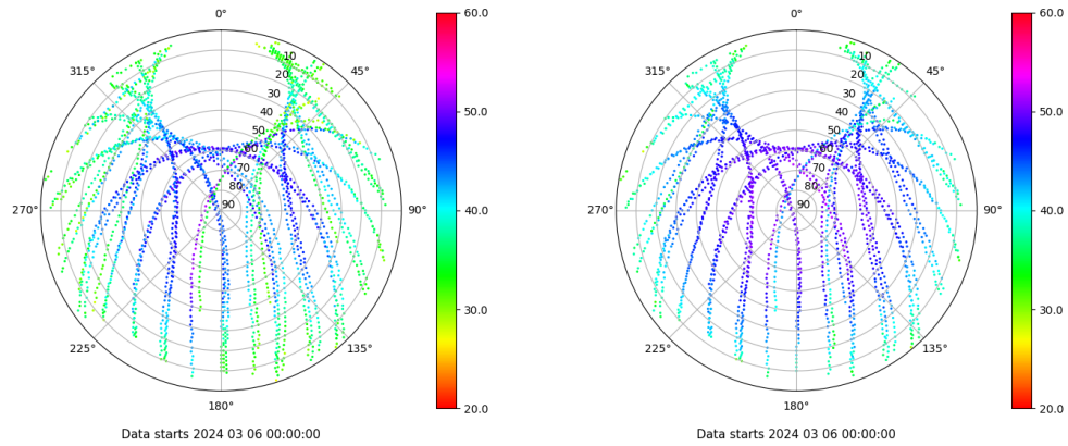
Skyplot for station ZARA. Signal to Noise S1C Data file ZARA00ESP_R_2024066.xtr Skyplot for station ZARA. Signal to Noise S2C Data file ZARA00ESP_R_2024066.xtr
