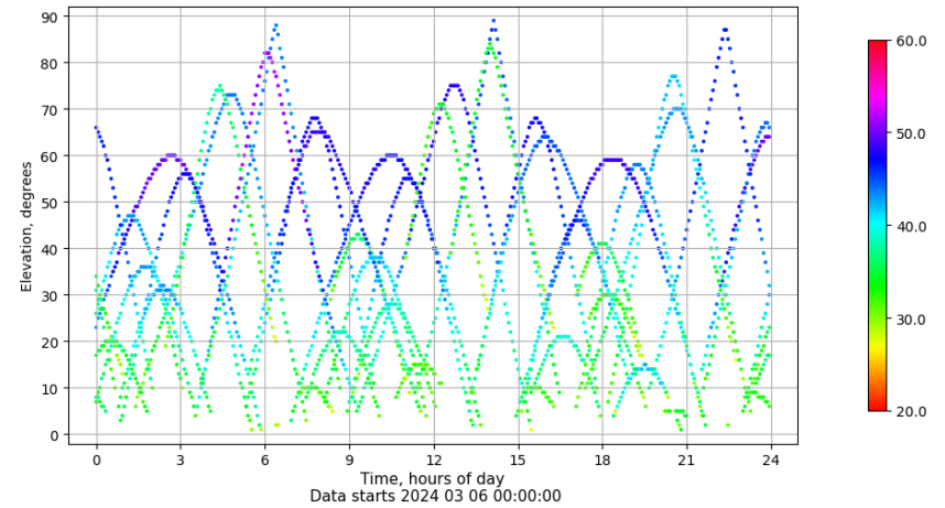
Time-elevation plot for station ZARA. Signal to Noise S1C Data file ZARA00ESP_R_2024066.xtr
