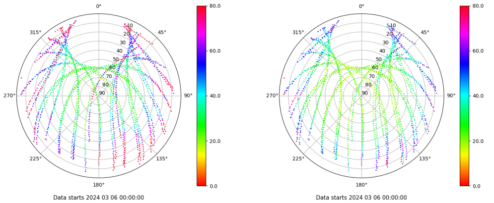
Skyplot for station ZARA. Parameter M1C Data file ZARA00ESP_R_2024066.xtr Skyplot for station ZARA. Parameter M2C Data file ZARA00ESP_R_2024066.xtr
