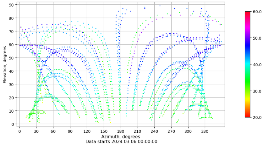
Azimuth-elevation plot for station ZARA. Signal to Noise S1C Data file ZARA00ESP_R_2024066.xtr
