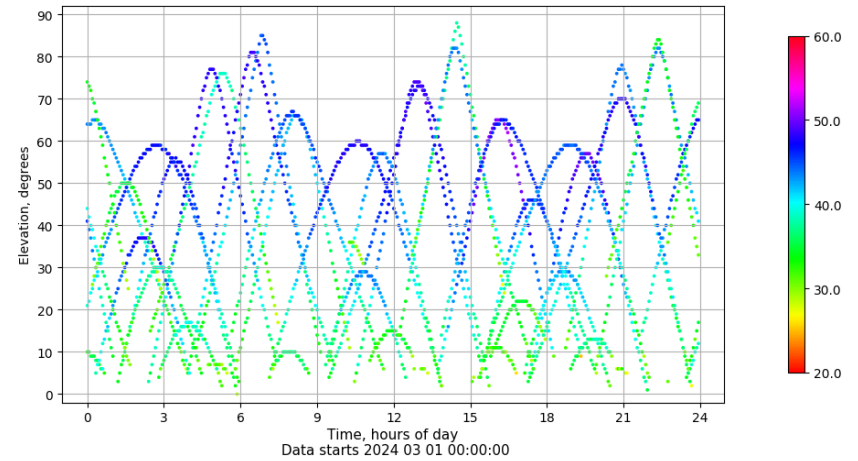
Time-elevation plot for station ZARA. Signal to Noise S1C Data file ZARA00ESP_R_2024061.xtr
