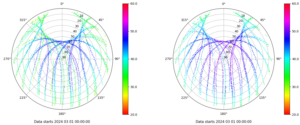
Skyplot for station ZARA. Signal to Noise S1C Data file ZARA00ESP_R_2024061.xtr Skyplot for station ZARA. Signal to Noise S2C Data file ZARA00ESP_R_2024061.xtr
