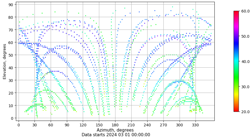
Azimuth-elevation plot for station ZARA. Signal to Noise S1C Data file ZARA00ESP_R_2024061.xtr
