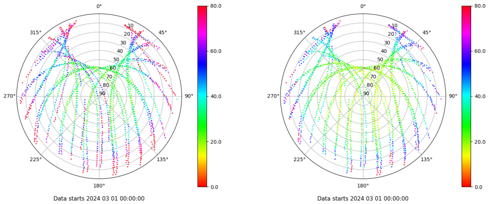
Skyplot for station ZARA. Parameter M1C Data file ZARA00ESP_R_2024061.xtr Skyplot for station ZARA. Parameter M2C Data file ZARA00ESP_R_2024061.xtr
