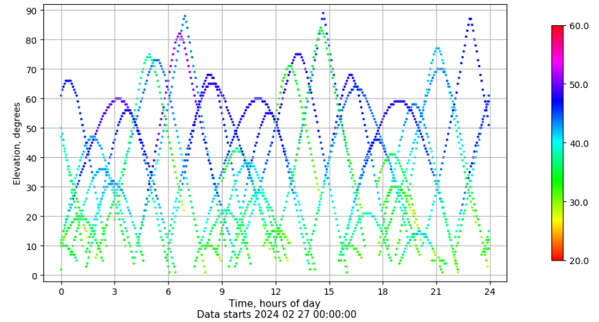
Time-elevation plot for station ZARA. Signal to Noise S1C Data file ZARA00ESP_R_2024058.xtr
