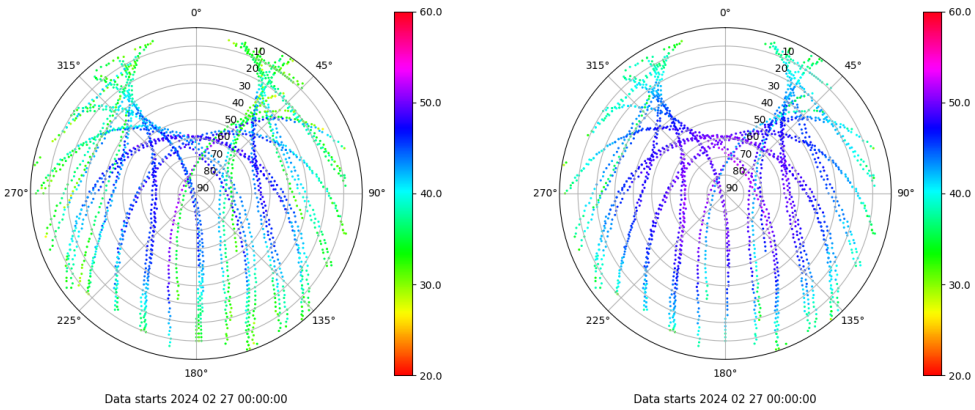
Skyplot for station ZARA. Signal to Noise S1C Data file ZARA00ESP_R_2024058.xtr Skyplot for station ZARA. Signal to Noise S2C Data file ZARA00ESP_R_2024058.xtr
