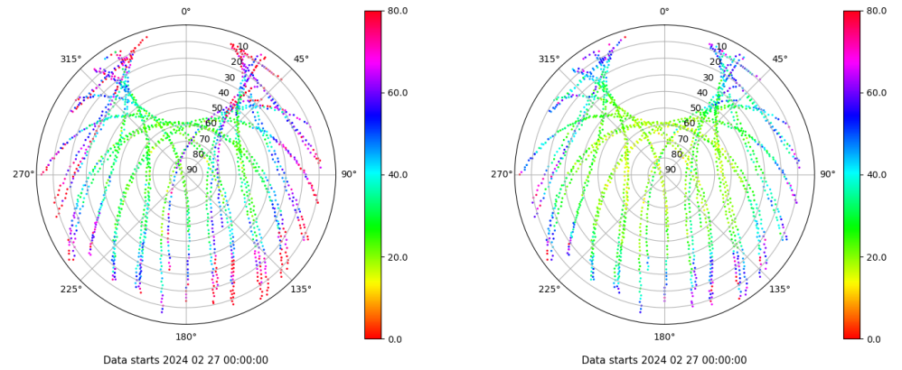
Skyplot for station ZARA. Parameter M1C Data file ZARA00ESP_R_2024058.xtr Skyplot for station ZARA. Parameter M2C Data file ZARA00ESP_R_2024058.xtr
