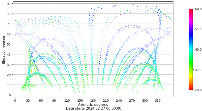
Azimuth-elevation plot for station ZARA. Signal to Noise S1C Data file ZARA00ESP_R_2024058.xtr
