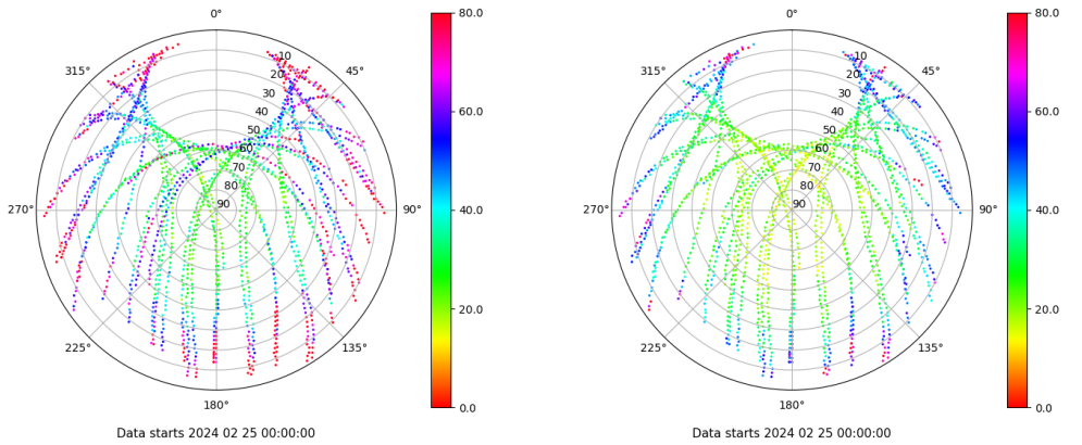
Skyplot for station ZARA. Parameter M1C Data file ZARA00ESP_R_2024056.xtr Skyplot for station ZARA. Parameter M2C Data file ZARA00ESP_R_2024056.xtr
