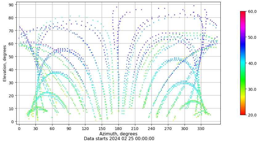
Azimuth-elevation plot for station ZARA. Signal to Noise S1C Data file ZARA00ESP_R_2024056.xtr
