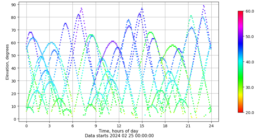
Time-elevation plot for station ZARA. Signal to Noise S1C Data file ZARA00ESP_R_2024056.xtr
