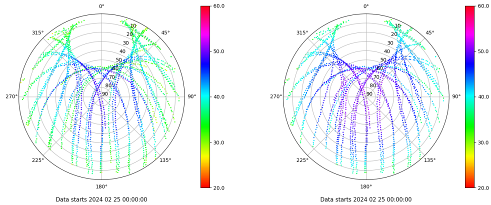
Skyplot for station ZARA. Signal to Noise S1C Data file ZARA00ESP_R_2024056.xtr Skyplot for station ZARA. Signal to Noise S2C Data file ZARA00ESP_R_2024056.xtr
