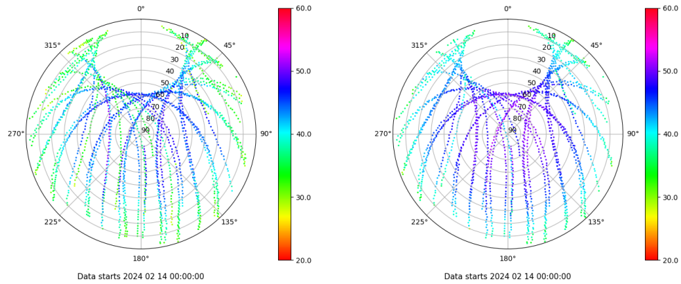
Skyplot for station ZARA. Signal to Noise S1C Data file ZARA00ESP_R_2024045.xtr Skyplot for station ZARA. Signal to Noise S2C Data file ZARA00ESP_R_2024045.xtr
