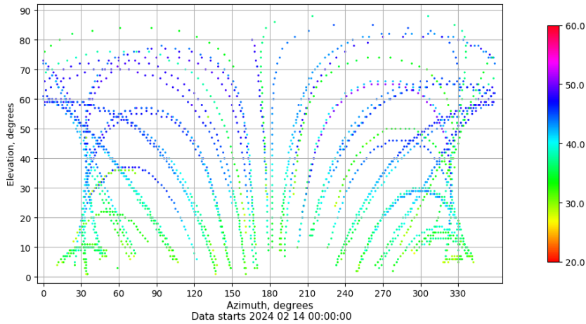
Azimuth-elevation plot for station ZARA. Signal to Noise S1C Data file ZARA00ESP_R_2024045.xtr
