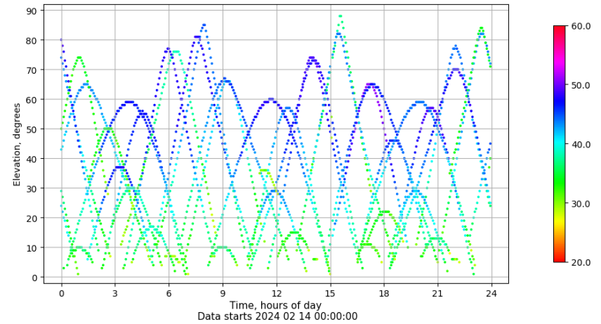
Time-elevation plot for station ZARA. Signal to Noise S1C Data file ZARA00ESP_R_2024045.xtr
