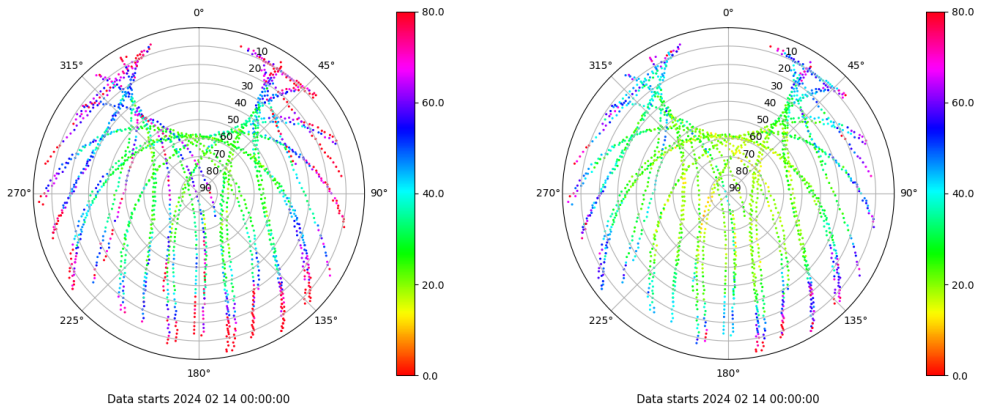
Skyplot for station ZARA. Parameter M1C Data file ZARA00ESP_R_2024045.xtr Skyplot for station ZARA. Parameter M2C Data file ZARA00ESP_R_2024045.xtr
