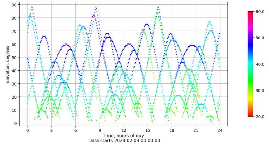
Time-elevation plot for station ZARA. Signal to Noise S1C Data file ZARA00ESP_R_2024034.xtr
