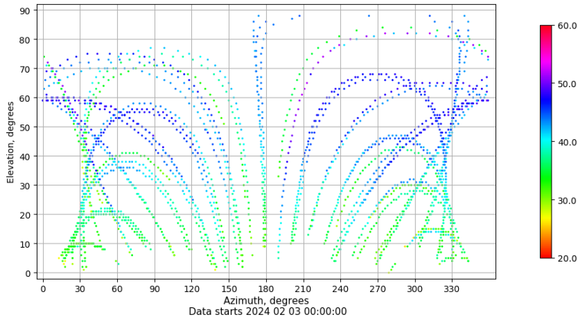
Azimuth-elevation plot for station ZARA. Signal to Noise S1C Data file ZARA00ESP_R_2024034.xtr
