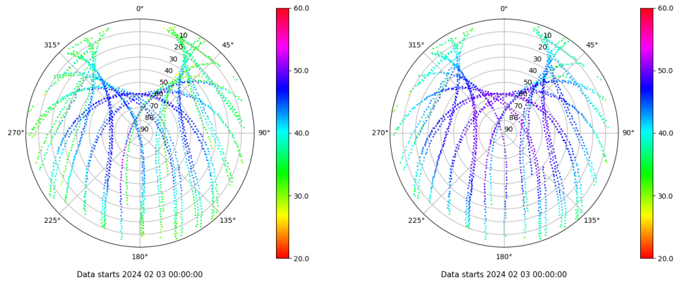
Skyplot for station ZARA. Signal to Noise S1C Data file ZARA00ESP_R_2024034.xtr Skyplot for station ZARA. Signal to Noise S2C Data file ZARA00ESP_R_2024034.xtr
