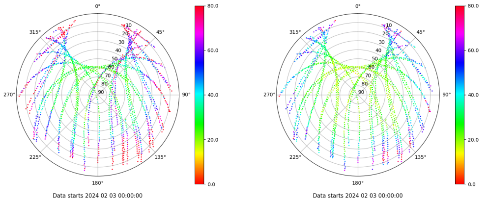
Skyplot for station ZARA. Parameter M1C Data file ZARA00ESP_R_2024034.xtr Skyplot for station ZARA. Parameter M2C Data file ZARA00ESP_R_2024034.xtr
