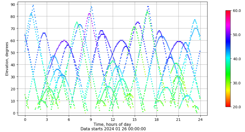
Time-elevation plot for station ZARA. Signal to Noise S1C Data file ZARA00ESP_R_2024026.xtr
