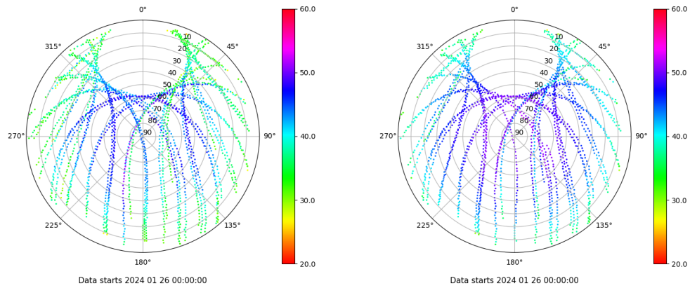
Skyplot for station ZARA. Signal to Noise S1C Data file ZARA00ESP_R_2024026.xtr Skyplot for station ZARA. Signal to Noise S2C Data file ZARA00ESP_R_2024026.xtr
