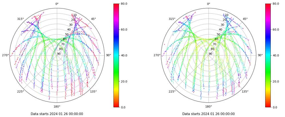
Skyplot for station ZARA. Parameter M1C Data file ZARA00ESP_R_2024026.xtr Skyplot for station ZARA. Parameter M2C Data file ZARA00ESP_R_2024026.xtr
