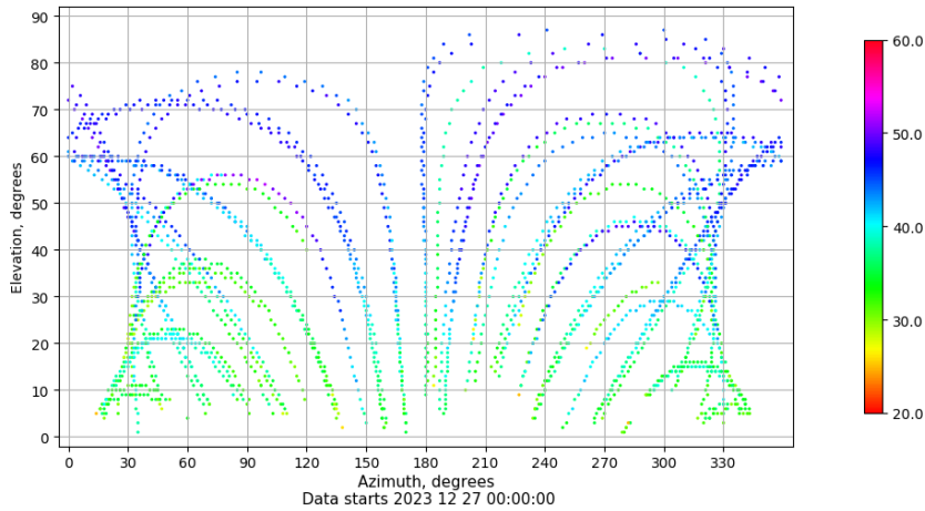
Azimuth-elevation plot for station ZARA. Signal to Noise S1C Data file ZARA00ESP_R_2023361.xtr
