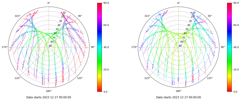
Skyplot for station ZARA. Parameter M1C Data file ZARA00ESP_R_2023361.xtr Skyplot for station ZARA. Parameter M2C Data file ZARA00ESP_R_2023361.xtr
