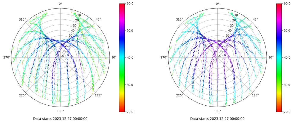
Skyplot for station ZARA. Signal to Noise S1C Data file ZARA00ESP_R_2023361.xtr Skyplot for station ZARA. Signal to Noise S2C Data file ZARA00ESP_R_2023361.xtr
