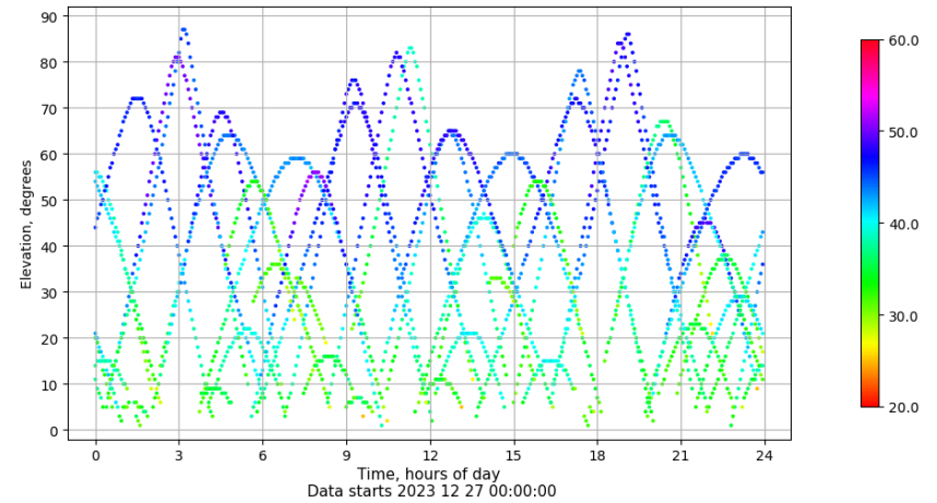
Time-elevation plot for station ZARA. Signal to Noise S1C Data file ZARA00ESP_R_2023361.xtr
