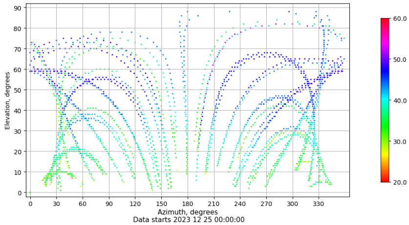
Azimuth-elevation plot for station ZARA. Signal to Noise S1C Data file ZARA00ESP_R_2023359.xtr
