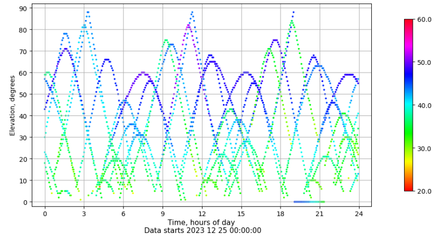
Time-elevation plot for station ZARA. Signal to Noise S1C Data file ZARA00ESP_R_2023359.xtr
