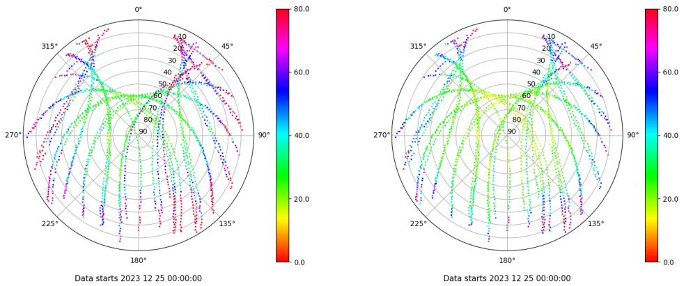
Skyplot for station ZARA. Parameter M1C Data file ZARA00ESP_R_2023359.xtr Skyplot for station ZARA. Parameter M2C Data file ZARA00ESP_R_2023359.xtr
