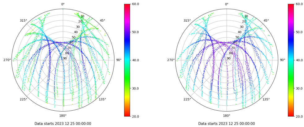
Skyplot for station ZARA. Signal to Noise S1C Data file ZARA00ESP_R_2023359.xtr Skyplot for station ZARA. Signal to Noise S2C Data file ZARA00ESP_R_2023359.xtr
