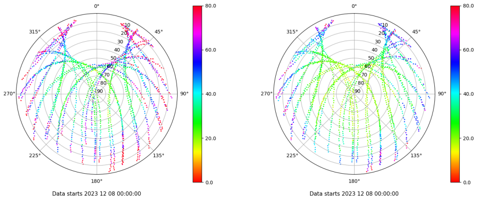
Skyplot for station ZARA. Parameter M1C Data file ZARA00ESP_R_2023342.xtr Skyplot for station ZARA. Parameter M2C Data file ZARA00ESP_R_2023342.xtr
