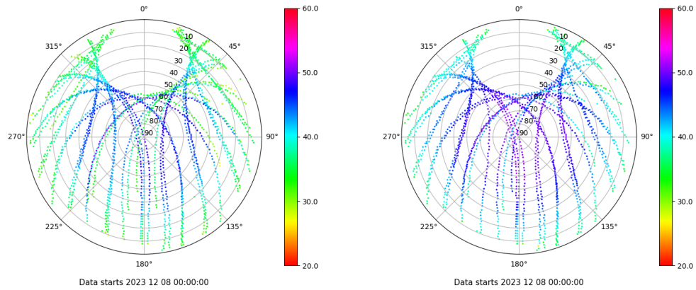
Skyplot for station ZARA. Signal to Noise S1C Data file ZARA00ESP_R_2023342.xtr Skyplot for station ZARA. Signal to Noise S2C Data file ZARA00ESP_R_2023342.xtr
