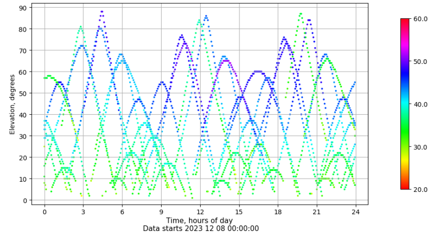
Time-elevation plot for station ZARA. Signal to Noise S1C Data file ZARA00ESP_R_2023342.xtr
