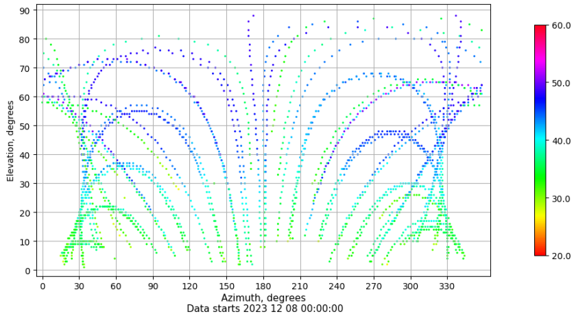
Azimuth-elevation plot for station ZARA. Signal to Noise S1C Data file ZARA00ESP_R_2023342.xtr
