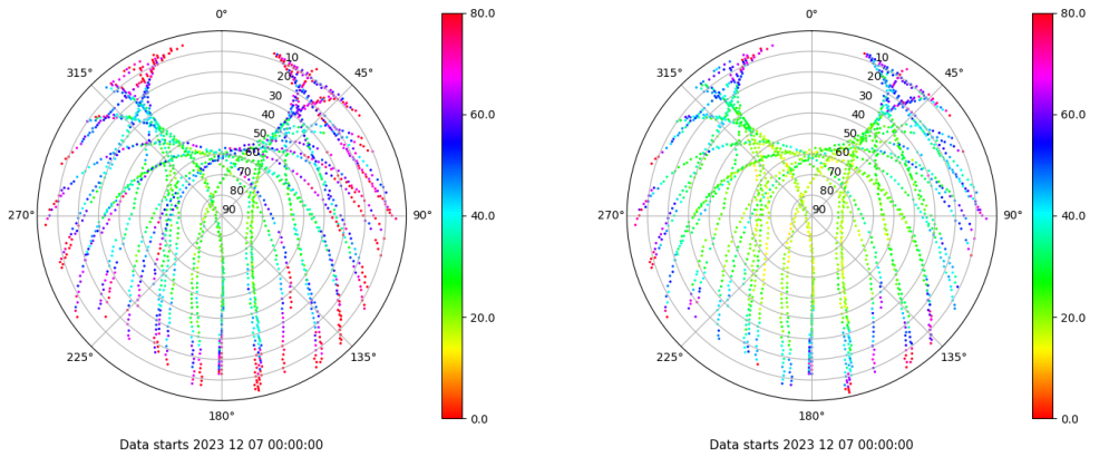
Skyplot for station ZARA. Parameter M1C Data file ZARA00ESP_R_2023341.xtr Skyplot for station ZARA. Parameter M2C Data file ZARA00ESP_R_2023341.xtr
