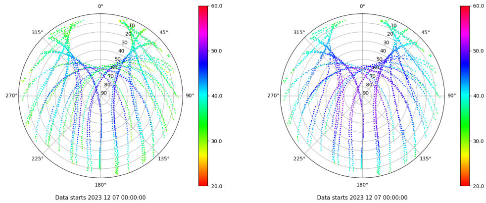
Skyplot for station ZARA. Signal to Noise S1C Data file ZARA00ESP_R_2023341.xtr Skyplot for station ZARA. Signal to Noise S2C Data file ZARA00ESP_R_2023341.xtr
