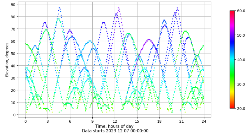
Time-elevation plot for station ZARA. Signal to Noise S1C Data file ZARA00ESP_R_2023341.xtr
