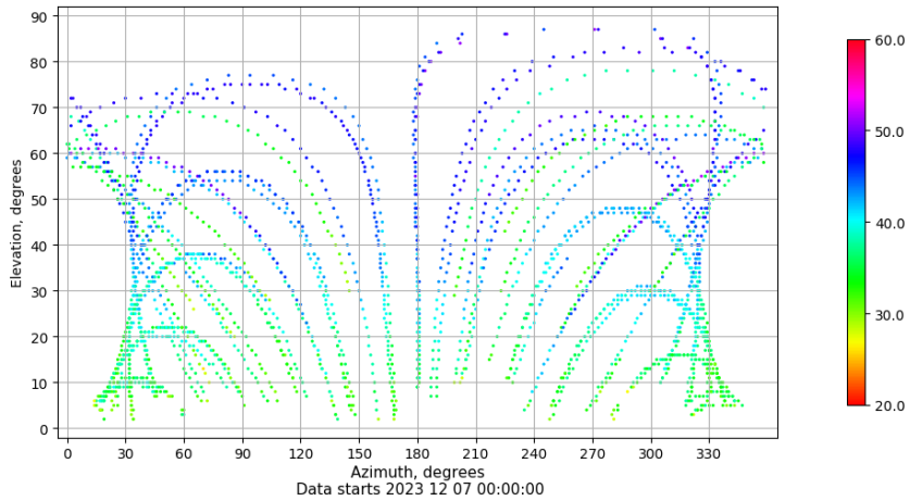
Azimuth-elevation plot for station ZARA. Signal to Noise S1C Data file ZARA00ESP_R_2023341.xtr
