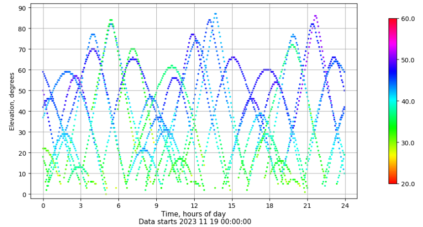
Time-elevation plot for station ZARA. Signal to Noise S1C Data file ZARA00ESP_R_2023323.xtr
