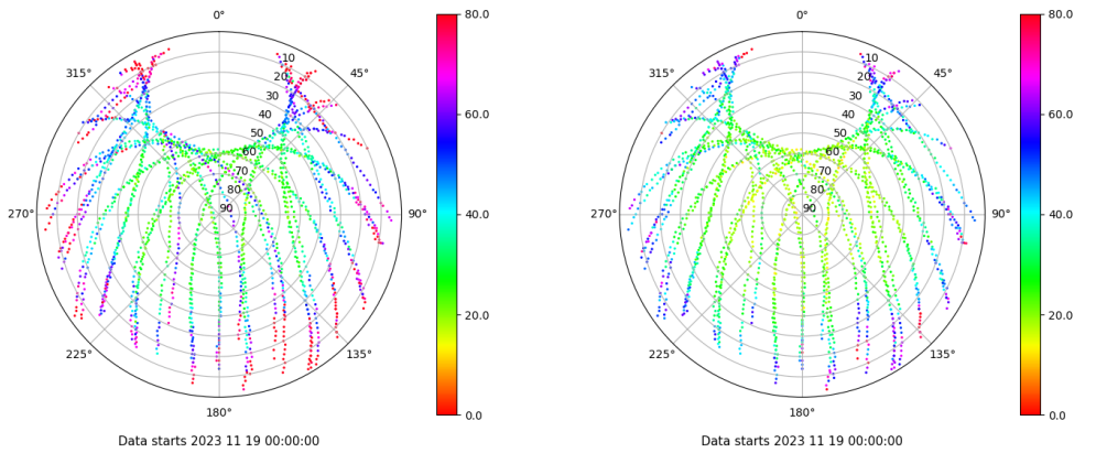
Skyplot for station ZARA. Parameter M1C Data file ZARA00ESP_R_2023323.xtr Skyplot for station ZARA. Parameter M2C Data file ZARA00ESP_R_2023323.xtr
