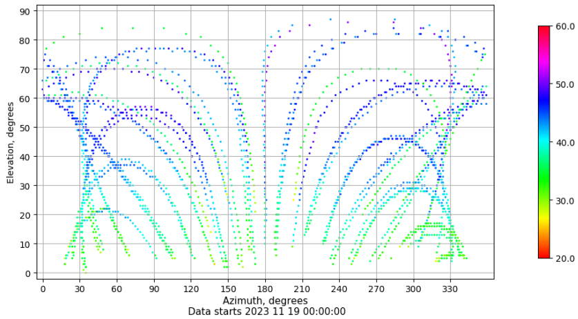
Azimuth-elevation plot for station ZARA. Signal to Noise S1C Data file ZARA00ESP_R_2023323.xtr
