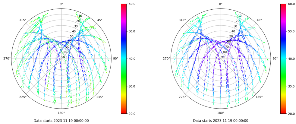
Skyplot for station ZARA. Signal to Noise S1C Data file ZARA00ESP_R_2023323.xtr Skyplot for station ZARA. Signal to Noise S2C Data file ZARA00ESP_R_2023323.xtr
