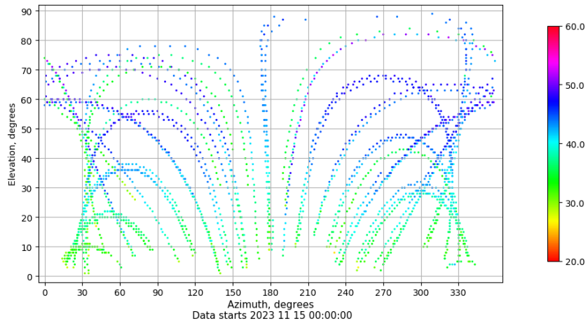
Azimuth-elevation plot for station ZARA. Signal to Noise S1C Data file ZARA00ESP_R_2023319.xtr
