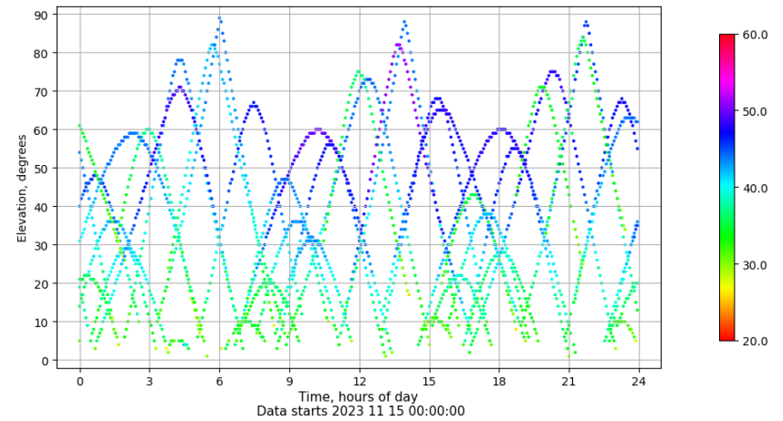
Time-elevation plot for station ZARA. Signal to Noise S1C Data file ZARA00ESP_R_2023319.xtr
