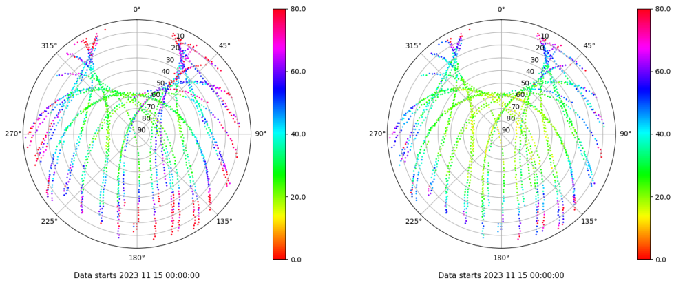
Skyplot for station ZARA. Parameter M1C Data file ZARA00ESP_R_2023319.xtr Skyplot for station ZARA. Parameter M2C Data file ZARA00ESP_R_2023319.xtr
