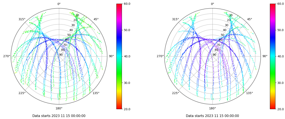
Skyplot for station ZARA. Signal to Noise S1C Data file ZARA00ESP_R_2023319.xtr Skyplot for station ZARA. Signal to Noise S2C Data file ZARA00ESP_R_2023319.xtr
