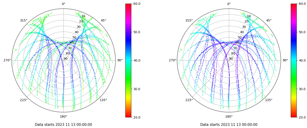
Skyplot for station ZARA. Signal to Noise S1C Data file ZARA00ESP_R_2023317.xtr Skyplot for station ZARA. Signal to Noise S2C Data file ZARA00ESP_R_2023317.xtr
