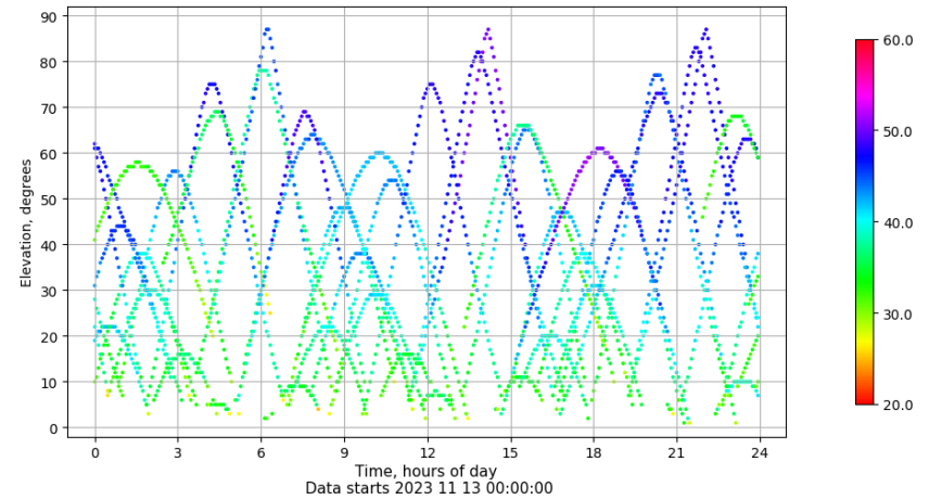
Time-elevation plot for station ZARA. Signal to Noise S1C Data file ZARA00ESP_R_2023317.xtr
