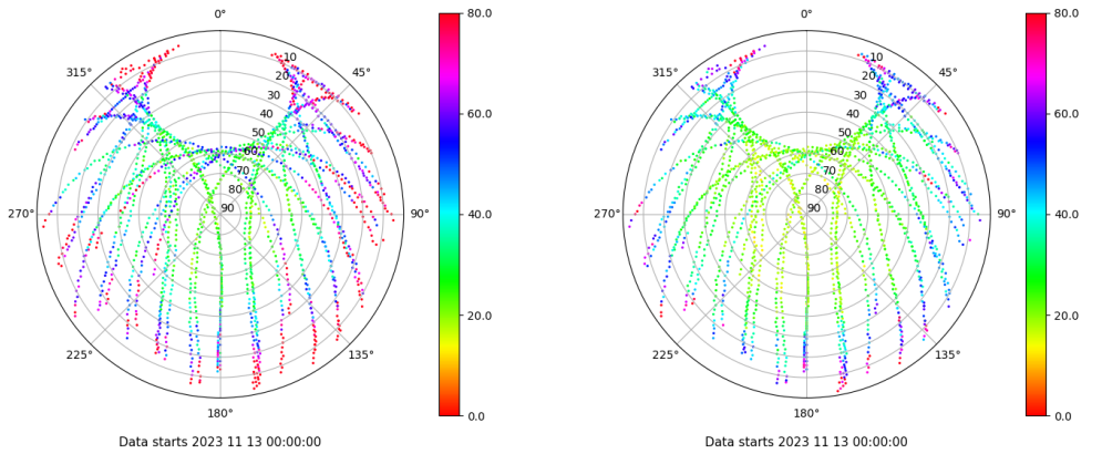
Skyplot for station ZARA. Parameter M1C Data file ZARA00ESP_R_2023317.xtr Skyplot for station ZARA. Parameter M2C Data file ZARA00ESP_R_2023317.xtr
