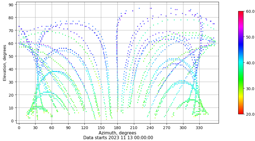
Azimuth-elevation plot for station ZARA. Signal to Noise S1C Data file ZARA00ESP_R_2023317.xtr
