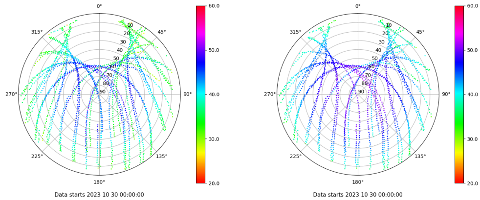
Skyplot for station ZARA. Signal to Noise S1C Data file ZARA00ESP_R_2023303.xtr Skyplot for station ZARA. Signal to Noise S2C Data file ZARA00ESP_R_2023303.xtr
