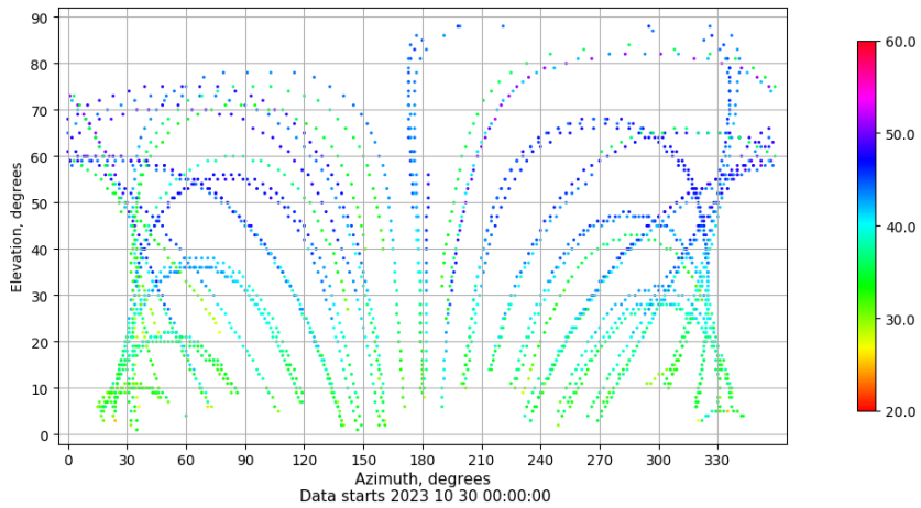
Azimuth-elevation plot for station ZARA. Signal to Noise S1C Data file ZARA00ESP_R_2023303.xtr
