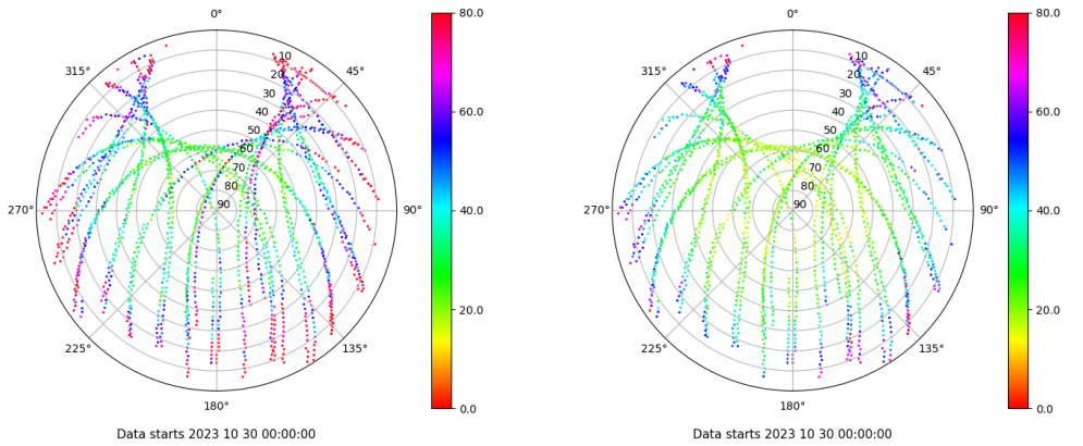
Skyplot for station ZARA. Parameter M1C Data file ZARA00ESP_R_2023303.xtr Skyplot for station ZARA. Parameter M2C Data file ZARA00ESP_R_2023303.xtr
