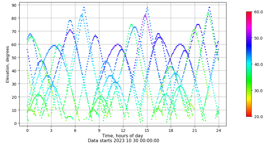
Time-elevation plot for station ZARA. Signal to Noise S1C Data file ZARA00ESP_R_2023303.xtr
