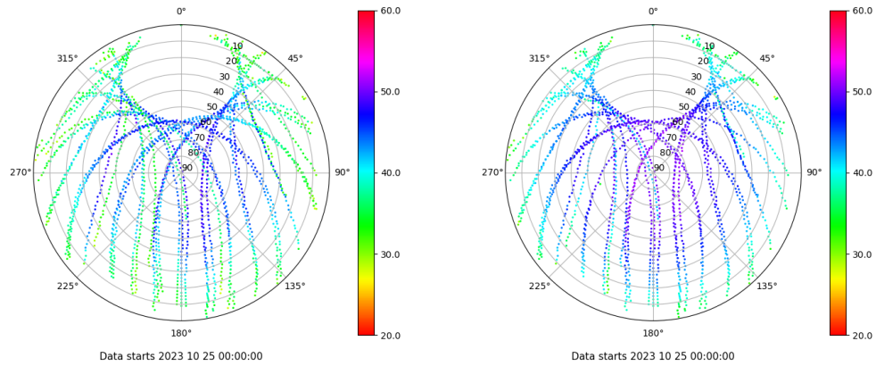
Skyplot for station ZARA. Signal to Noise S1C Data file ZARA00ESP_R_2023298.xtr Skyplot for station ZARA. Signal to Noise S2C Data file ZARA00ESP_R_2023298.xtr
