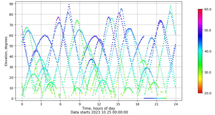
Time-elevation plot for station ZARA. Signal to Noise S1C Data file ZARA00ESP_R_2023298.xtr
