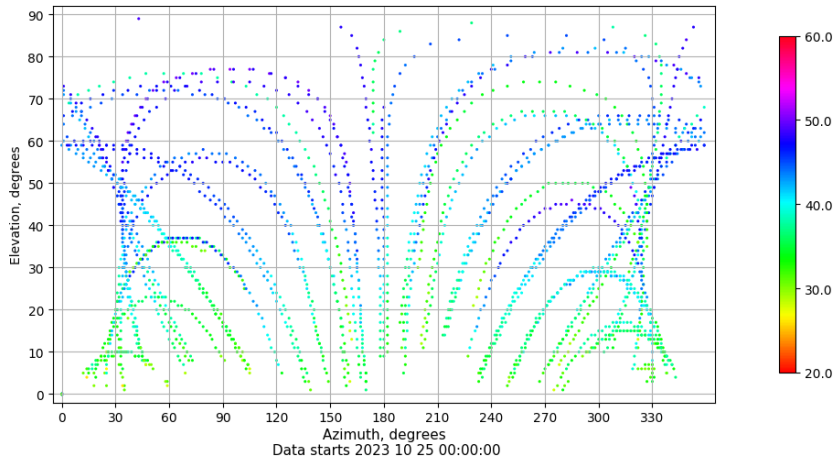
Azimuth-elevation plot for station ZARA. Signal to Noise S1C Data file ZARA00ESP_R_2023298.xtr
