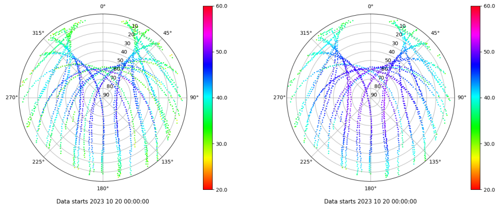
Skyplot for station ZARA. Signal to Noise S1C Data file ZARA00ESP_R_2023293.xtr Skyplot for station ZARA. Signal to Noise S2C Data file ZARA00ESP_R_2023293.xtr
