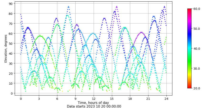
Time-elevation plot for station ZARA. Signal to Noise S1C Data file ZARA00ESP_R_2023293.xtr
