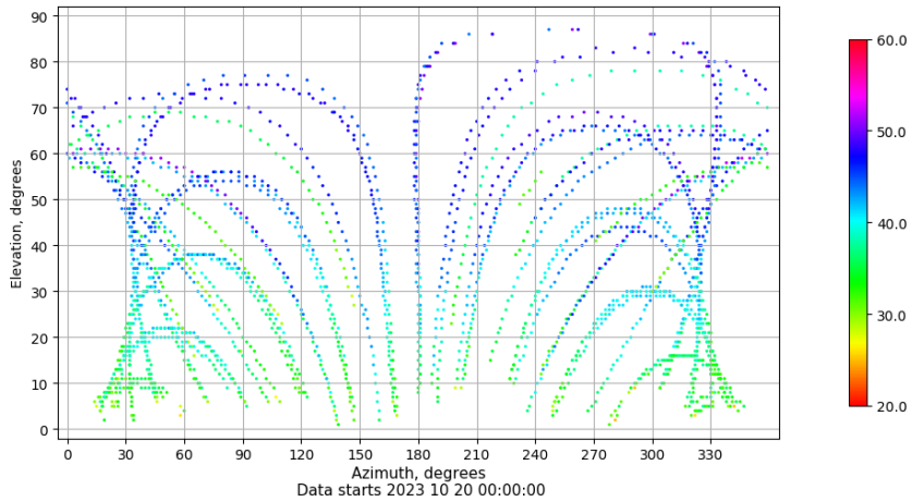
Azimuth-elevation plot for station ZARA. Signal to Noise S1C Data file ZARA00ESP_R_2023293.xtr
