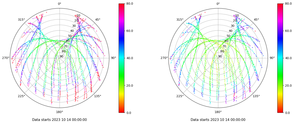
Skyplot for station ZARA. Parameter M1C Data file ZARA00ESP_R_2023287.xtr Skyplot for station ZARA. Parameter M2C Data file ZARA00ESP_R_2023287.xtr
