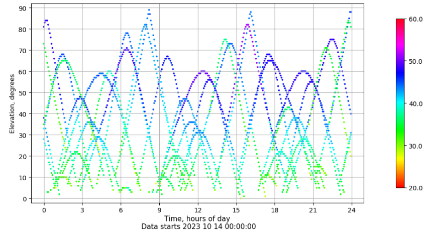
Time-elevation plot for station ZARA. Signal to Noise S1C Data file ZARA00ESP_R_2023287.xtr
