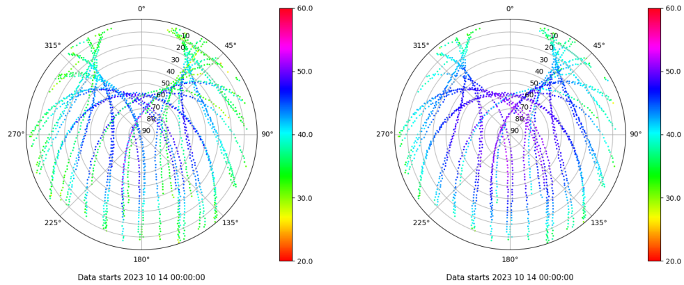
Skyplot for station ZARA. Signal to Noise S1C Data file ZARA00ESP_R_2023287.xtr Skyplot for station ZARA. Signal to Noise S2C Data file ZARA00ESP_R_2023287.xtr
