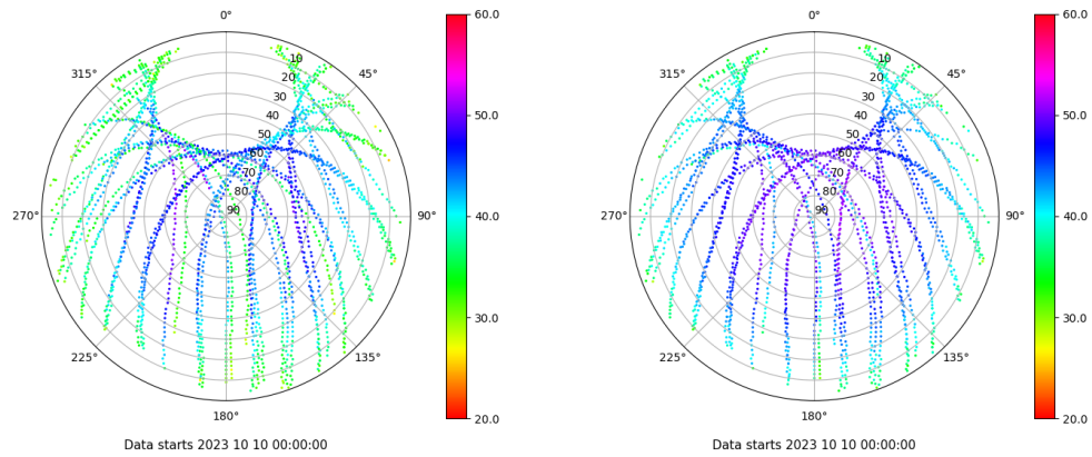
Skyplot for station ZARA. Signal to Noise S1C Data file ZARA00ESP_R_2023283.xtr Skyplot for station ZARA. Signal to Noise S2C Data file ZARA00ESP_R_2023283.xtr
