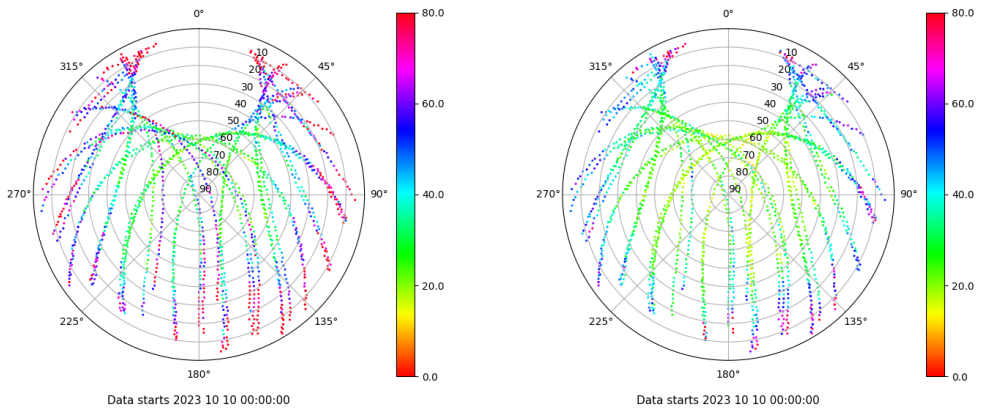
Skyplot for station ZARA. Parameter M1C Data file ZARA00ESP_R_2023283.xtr Skyplot for station ZARA. Parameter M2C Data file ZARA00ESP_R_2023283.xtr
