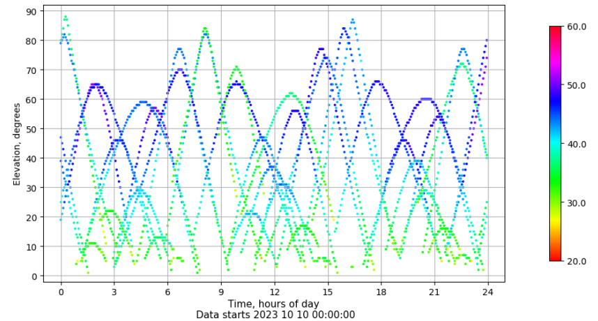
Time-elevation plot for station ZARA. Signal to Noise S1C Data file ZARA00ESP_R_2023283.xtr
