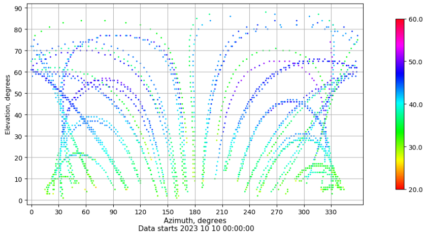
Azimuth-elevation plot for station ZARA. Signal to Noise S1C Data file ZARA00ESP_R_2023283.xtr
