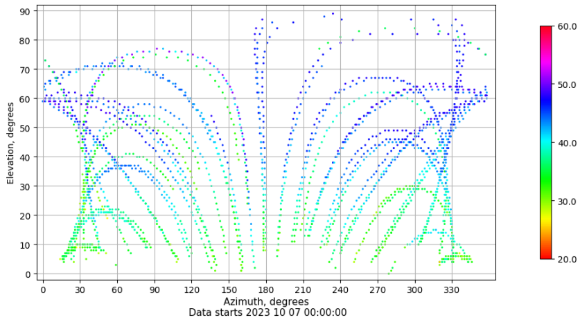
Azimuth-elevation plot for station ZARA. Signal to Noise S1C Data file ZARA00ESP_R_2023280.xtr
