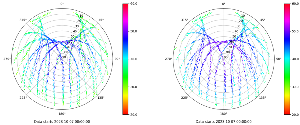
Skyplot for station ZARA. Signal to Noise S1C Data file ZARA00ESP_R_2023280.xtr Skyplot for station ZARA. Signal to Noise S2C Data file ZARA00ESP_R_2023280.xtr
