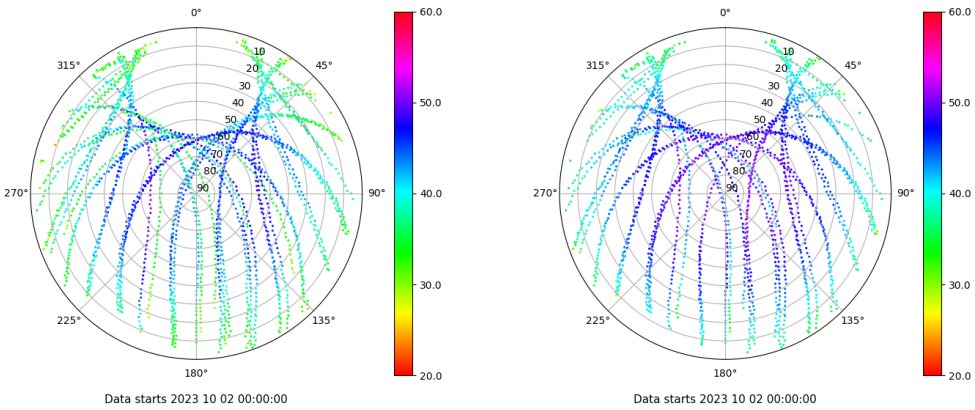
Skyplot for station ZARA. Signal to Noise S1C Data file ZARA00ESP_R_2023275.xtr Skyplot for station ZARA. Signal to Noise S2C Data file ZARA00ESP_R_2023275.xtr
