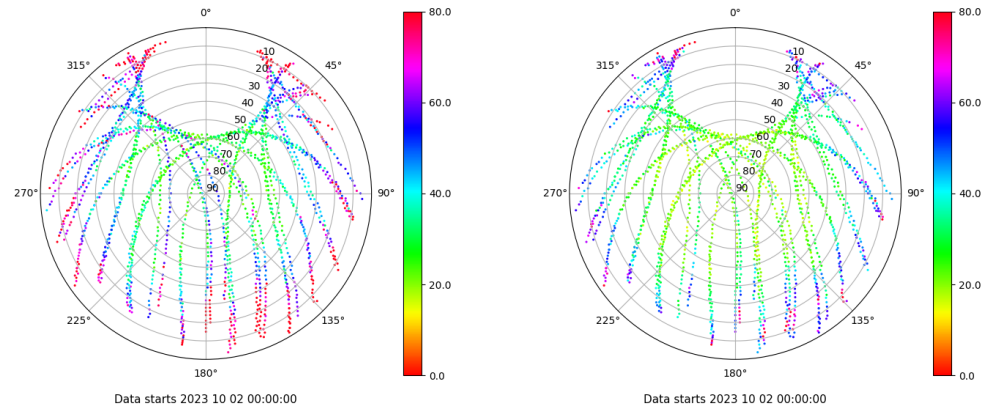
Skyplot for station ZARA. Parameter M1C Data file ZARA00ESP_R_2023275.xtr Skyplot for station ZARA. Parameter M2C Data file ZARA00ESP_R_2023275.xtr
