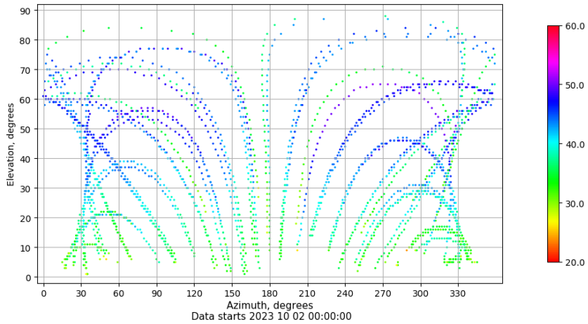
Azimuth-elevation plot for station ZARA. Signal to Noise S1C Data file ZARA00ESP_R_2023275.xtr
