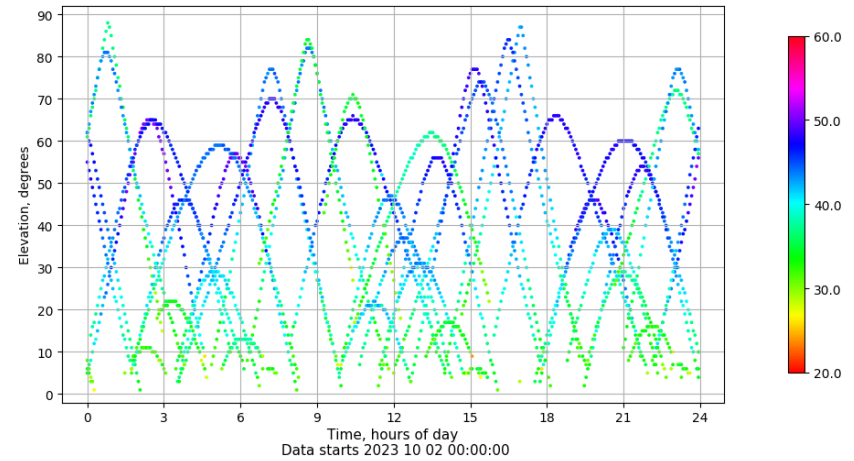
Time-elevation plot for station ZARA. Signal to Noise S1C Data file ZARA00ESP_R_2023275.xtr
