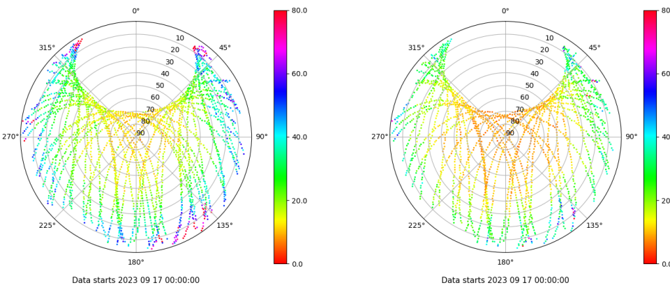
Skyplot for station ZARA. Parameter M1C Data file ZARA00ESP_R_2023260.xtr Skyplot for station ZARA. Parameter M2X Data file ZARA00ESP_R_2023260.xtr
