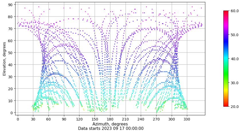
Azimuth-elevation plot for station ZARA. Signal to Noise S1C Data file ZARA00ESP_R_2023260.xtr
