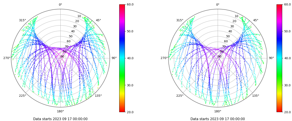
Skyplot for station ZARA. Signal to Noise S1C Data file ZARA00ESP_R_2023260.xtr Skyplot for station ZARA. Signal to Noise S2X Data file ZARA00ESP_R_2023260.xtr
