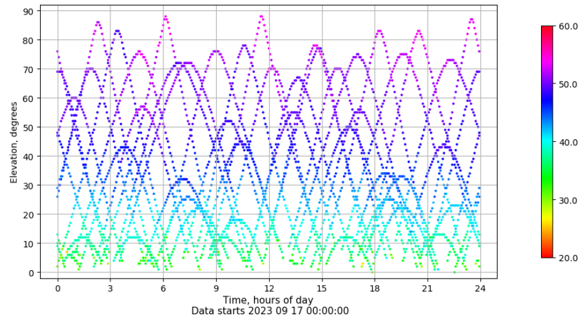
Time-elevation plot for station ZARA. Signal to Noise S1C Data file ZARA00ESP_R_2023260.xtr
