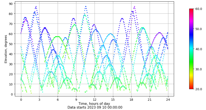
Time-elevation plot for station ZARA. Signal to Noise S1C Data file ZARA00ESP_R_2023253.xtr
