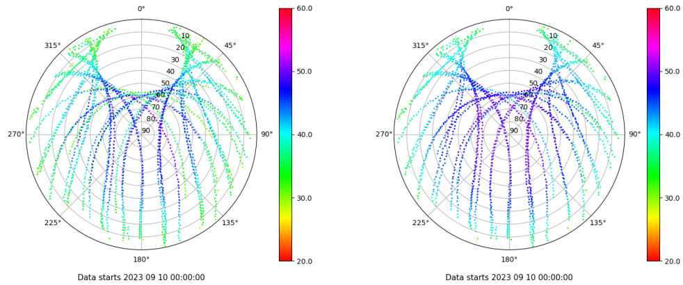
Skyplot for station ZARA. Signal to Noise S1C Data file ZARA00ESP_R_2023253.xtr Skyplot for station ZARA. Signal to Noise S2C Data file ZARA00ESP_R_2023253.xtr
