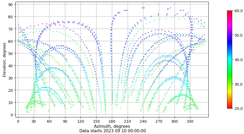
Azimuth-elevation plot for station ZARA. Signal to Noise S1C Data file ZARA00ESP_R_2023253.xtr
