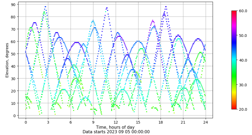
Time-elevation plot for station ZARA. Signal to Noise S1C Data file ZARA00ESP_R_2023248.xtr
