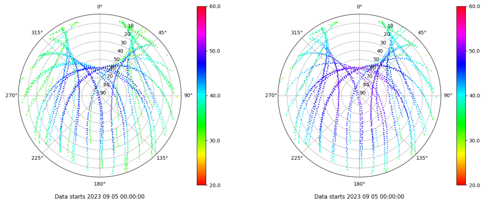
Skyplot for station ZARA. Signal to Noise S1C Data file ZARA00ESP_R_2023248.xtr Skyplot for station ZARA. Signal to Noise S2C Data file ZARA00ESP_R_2023248.xtr
