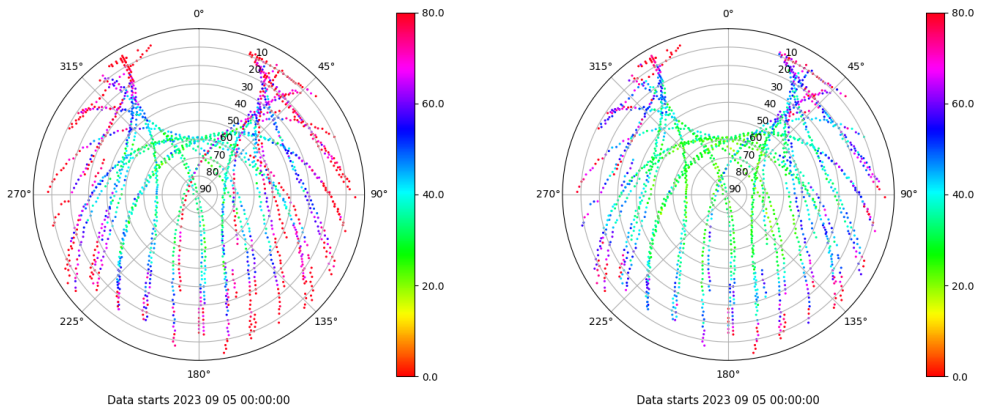
Skyplot for station ZARA. Parameter M1C Data file ZARA00ESP_R_2023248.xtr Skyplot for station ZARA. Parameter M2C Data file ZARA00ESP_R_2023248.xtr
