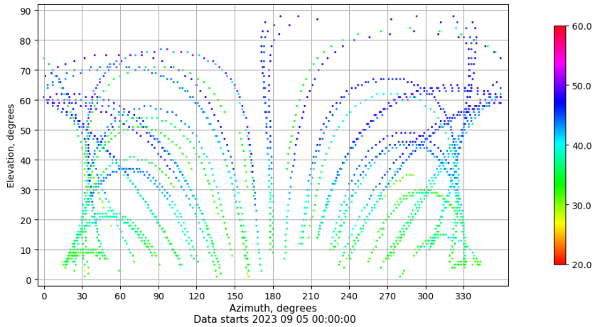
Azimuth-elevation plot for station ZARA. Signal to Noise S1C Data file ZARA00ESP_R_2023248.xtr
