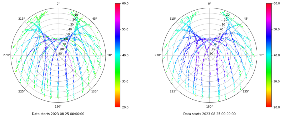
Skyplot for station ZARA. Signal to Noise S1C Data file ZARA00ESP_R_2023237.xtr Skyplot for station ZARA. Signal to Noise S2C Data file ZARA00ESP_R_2023237.xtr
