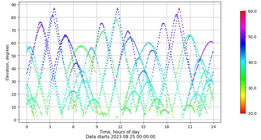
Time-elevation plot for station ZARA. Signal to Noise S1C Data file ZARA00ESP_R_2023237.xtr
