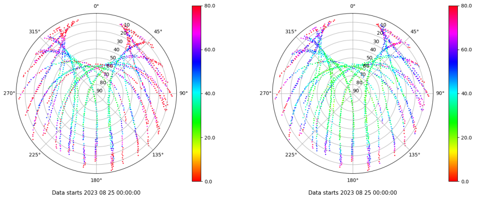
Skyplot for station ZARA. Parameter M1C Data file ZARA00ESP_R_2023237.xtr Skyplot for station ZARA. Parameter M2C Data file ZARA00ESP_R_2023237.xtr
