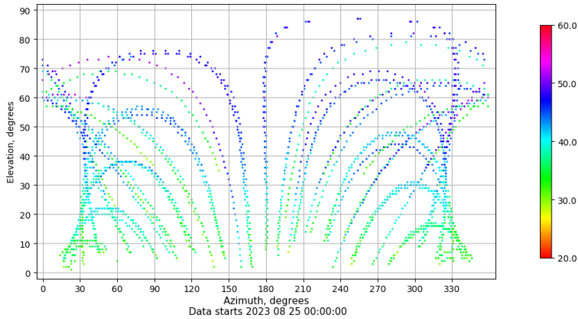
Azimuth-elevation plot for station ZARA. Signal to Noise S1C Data file ZARA00ESP_R_2023237.xtr
