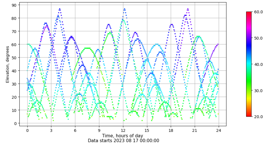
Time-elevation plot for station ZARA. Signal to Noise S1C Data file ZARA00ESP_R_2023229.xtr
