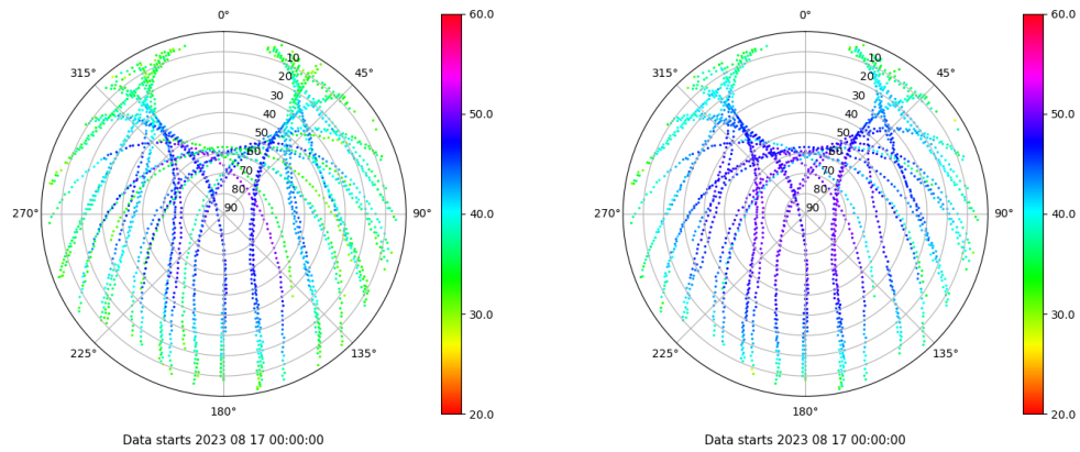
Skyplot for station ZARA. Signal to Noise S1C Data file ZARA00ESP_R_2023229.xtr Skyplot for station ZARA. Signal to Noise S2C Data file ZARA00ESP_R_2023229.xtr
