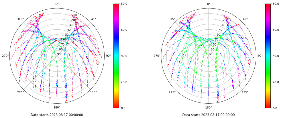
Skyplot for station ZARA. Parameter M1C Data file ZARA00ESP_R_2023229.xtr Skyplot for station ZARA. Parameter M2C Data file ZARA00ESP_R_2023229.xtr
