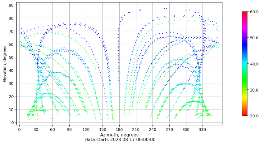
Azimuth-elevation plot for station ZARA. Signal to Noise S1C Data file ZARA00ESP_R_2023229.xtr
