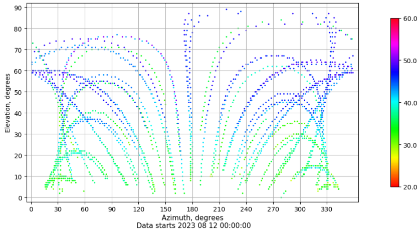
Azimuth-elevation plot for station ZARA. Signal to Noise S1C Data file ZARA00ESP_R_2023224.xtr
