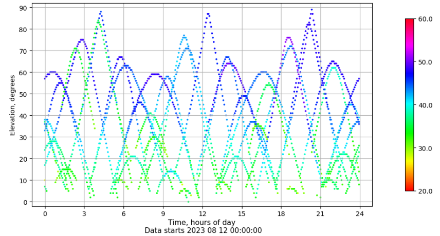
Time-elevation plot for station ZARA. Signal to Noise S1C Data file ZARA00ESP_R_2023224.xtr
