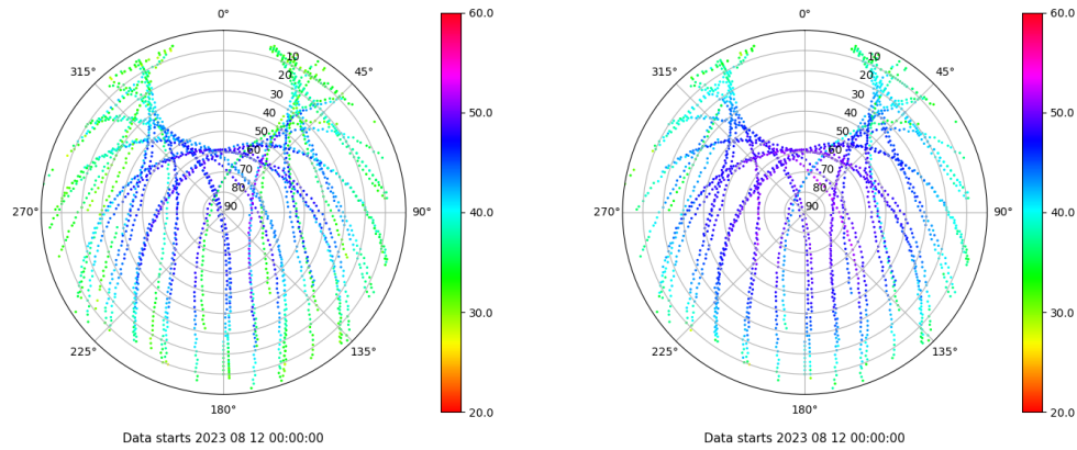
Skyplot for station ZARA. Signal to Noise S1C Data file ZARA00ESP_R_2023224.xtr Skyplot for station ZARA. Signal to Noise S2C Data file ZARA00ESP_R_2023224.xtr
