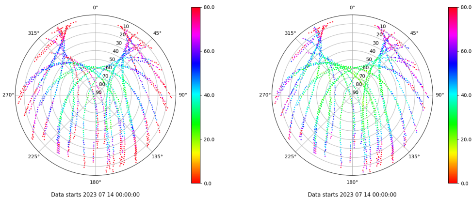
Skyplot for station ZARA. Parameter M1C Data file ZARA00ESP_R_2023195.xtr Skyplot for station ZARA. Parameter M2C Data file ZARA00ESP_R_2023195.xtr
