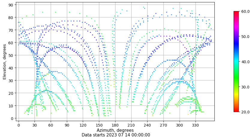
Azimuth-elevation plot for station ZARA. Signal to Noise S1C Data file ZARA00ESP_R_2023195.xtr
