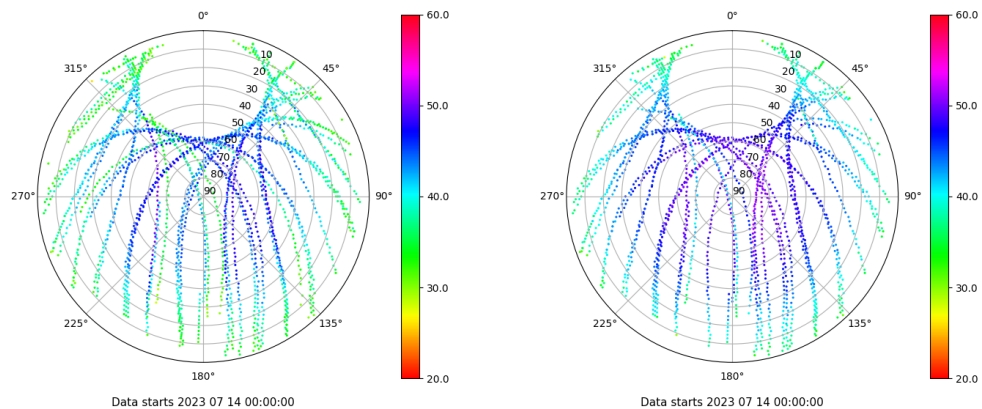
Skyplot for station ZARA. Signal to Noise S1C Data file ZARA00ESP_R_2023195.xtr Skyplot for station ZARA. Signal to Noise S2C Data file ZARA00ESP_R_2023195.xtr
