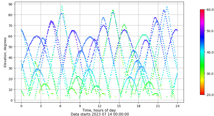
Time-elevation plot for station ZARA. Signal to Noise S1C Data file ZARA00ESP_R_2023195.xtr
